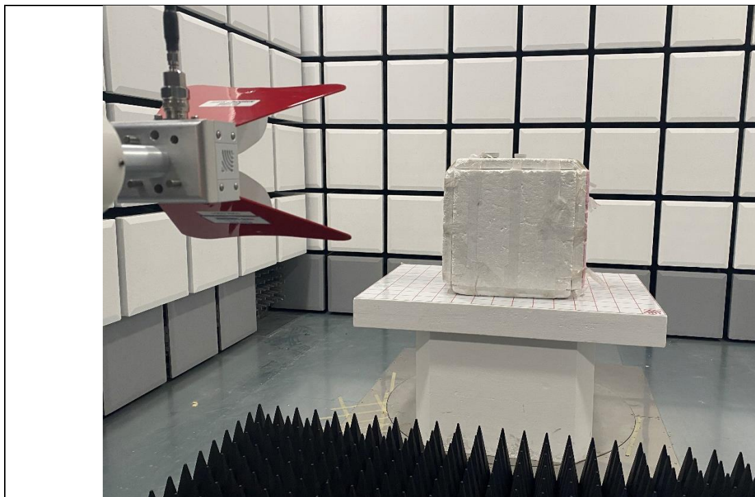
Radiated Emission Test above 1GHz Front View
