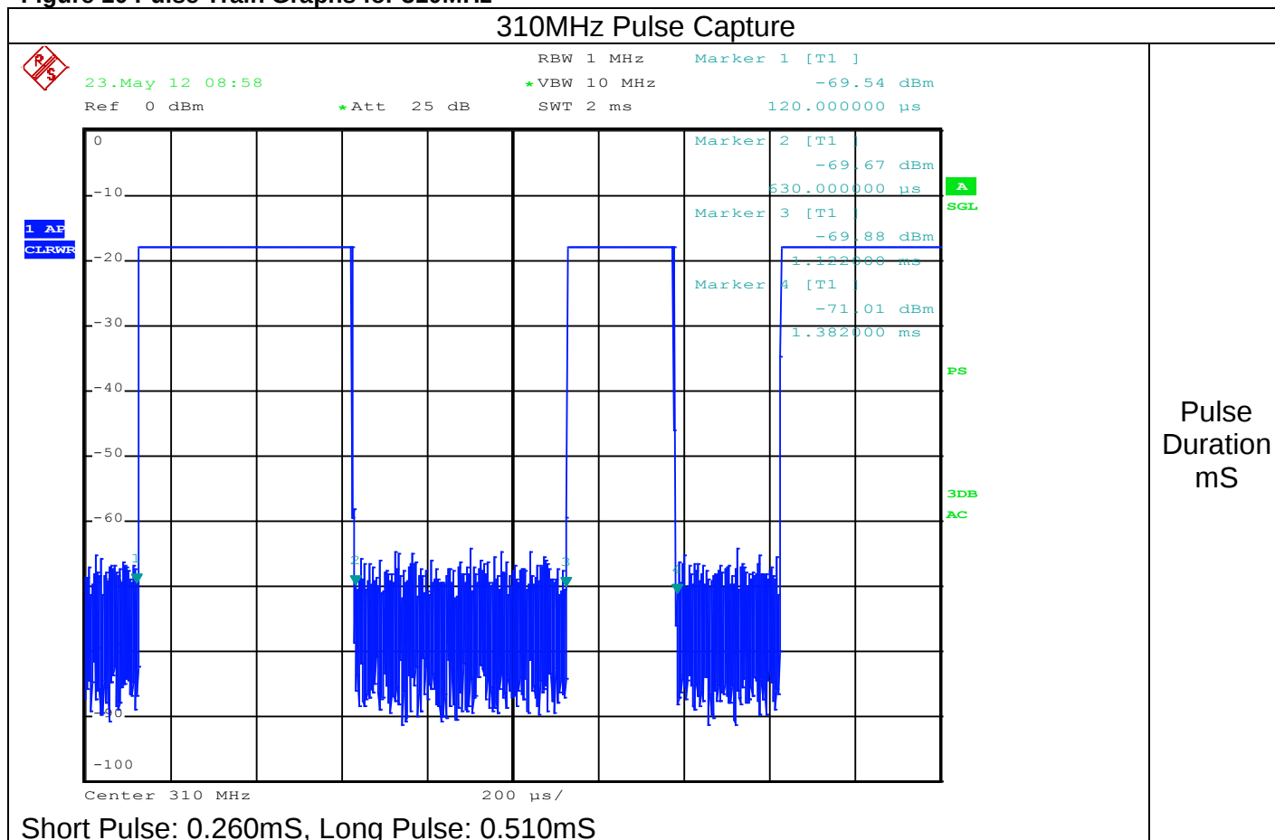
Figure 10 Pulse Train Graphs for 310MHz
