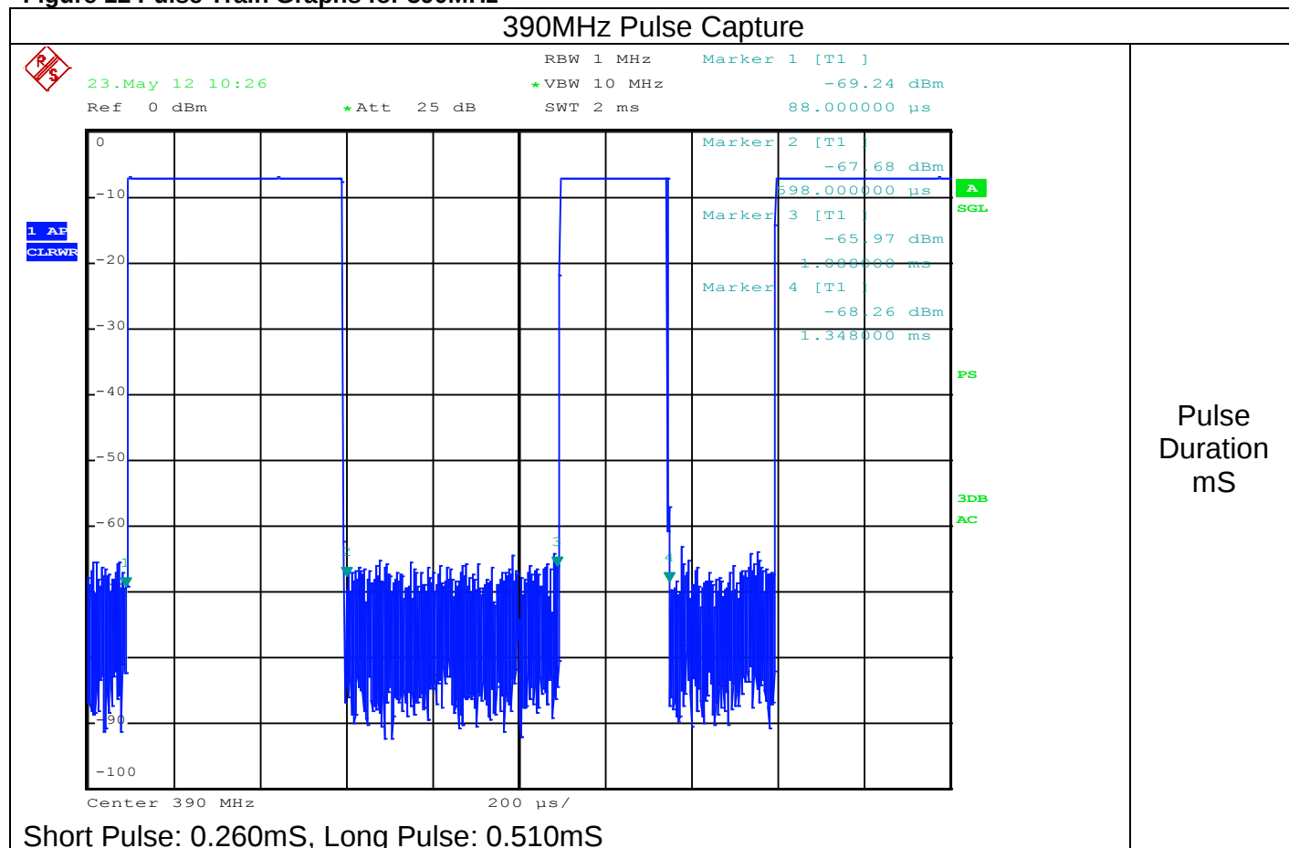
Figure 12 Pulse Train Graphs for 390MHz
