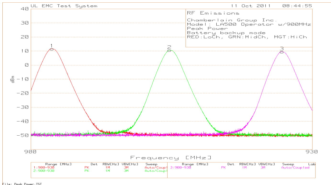
Figure 33 Maximum Peak Output Power Graph (Battery Mode)
