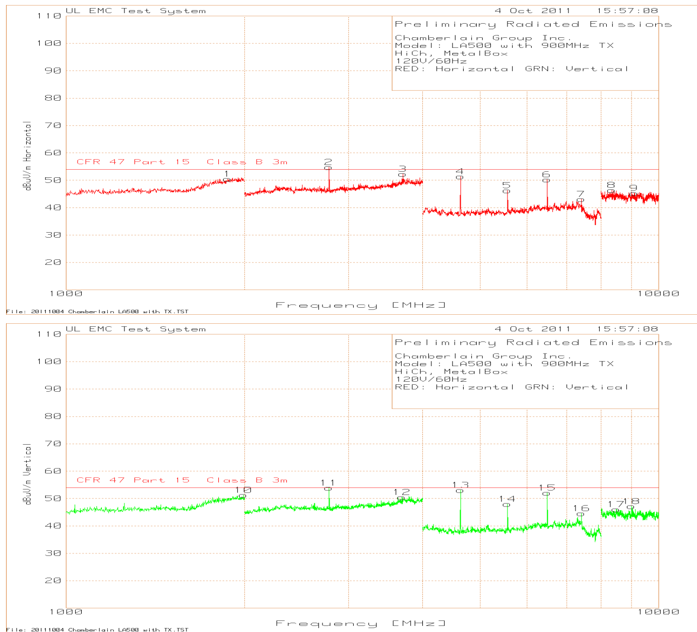
Figure 20 Radiated Spurious Emissions above 1GHz, High Channel (Metal Enclosure)
