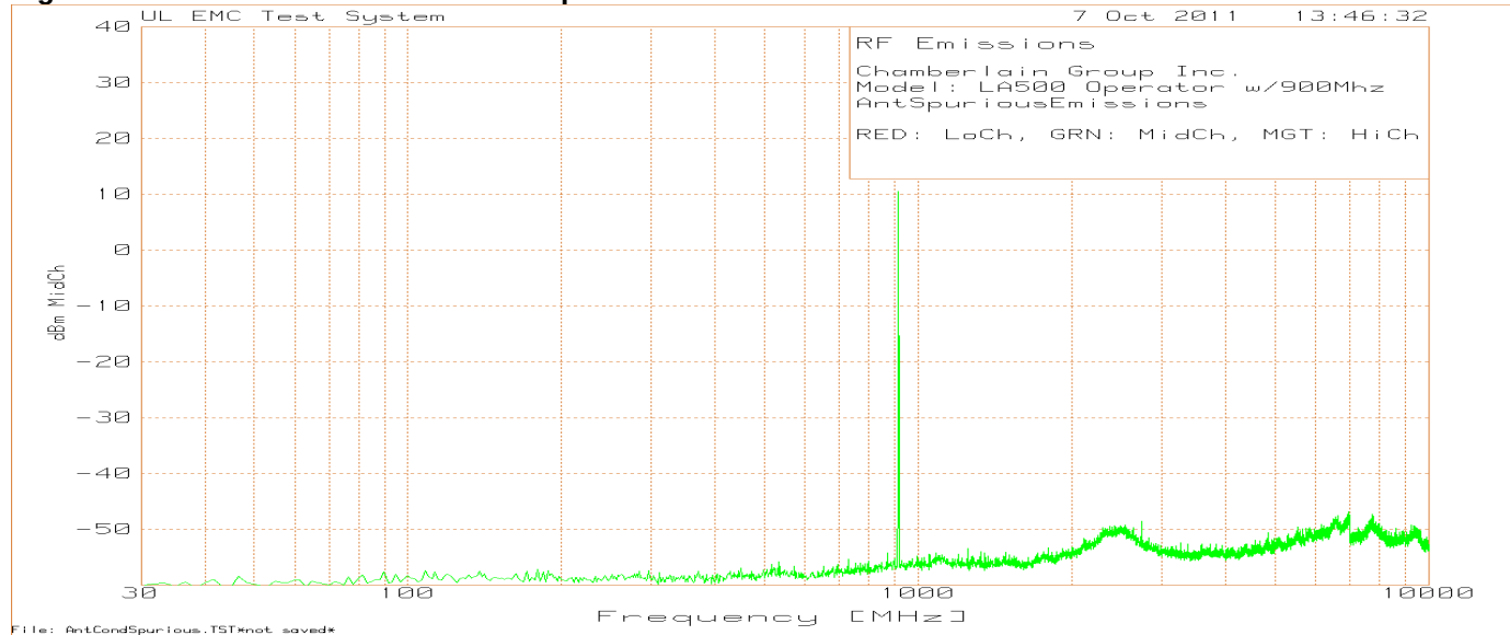
Figure 10 30MHz-10GHz Antenna Port Spurious Emissions Plots – Mid Channel
