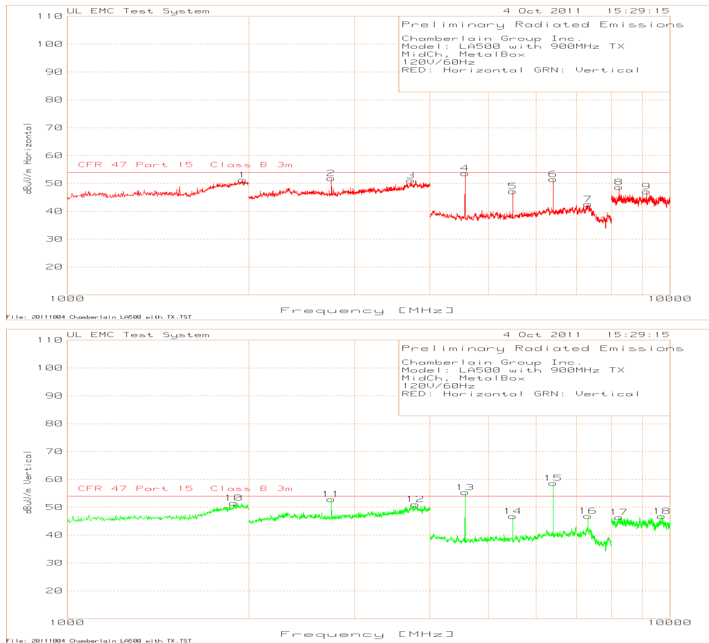
Figure 19 Radiated Spurious Emissions above 1GHz, Mid Channel (Metal Enclosure)
