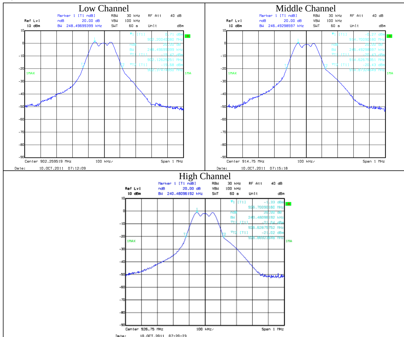
Figure 30 20dB Bandwidth Graphs
