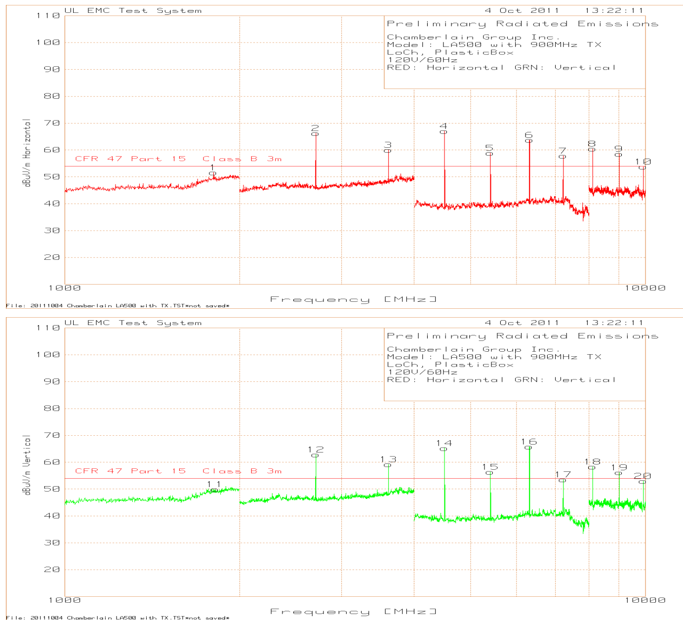
Figure 15 Radiated Spurious Emissions above 1GHz, Low Channel (Plastic Enclosure)
