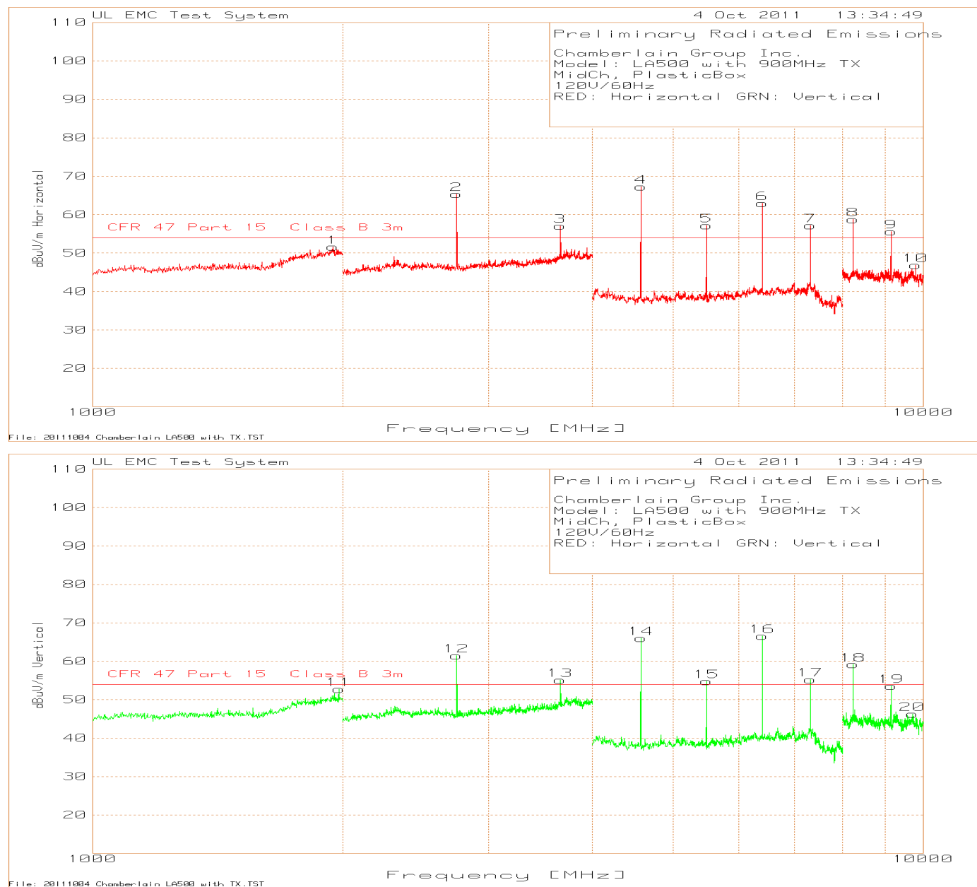
Figure 16 Radiated Spurious Emissions above 1GHz, Middle Channel (Plastic Enclosure)
