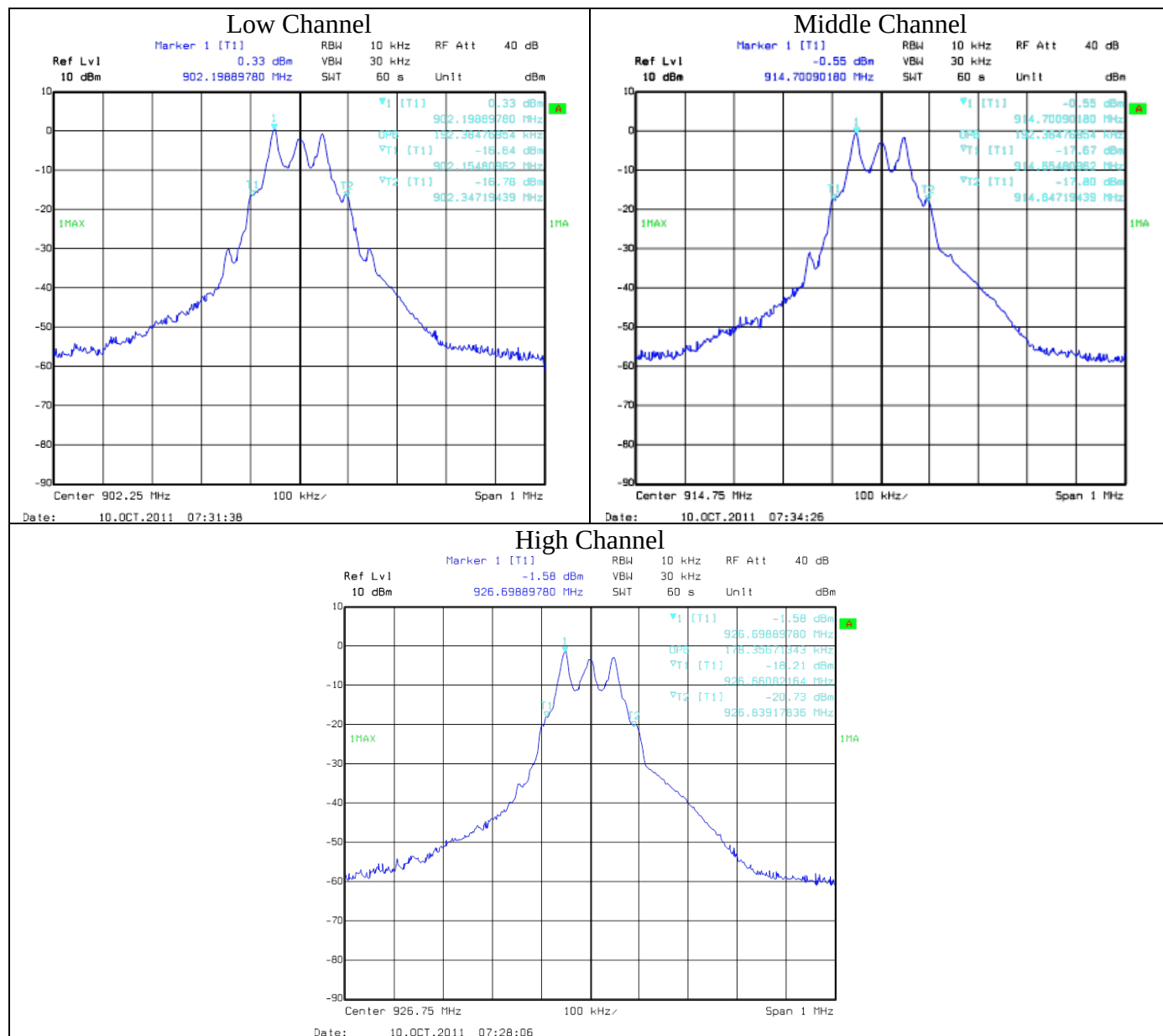
Figure 34 99% Power Bandwidth Graphs
