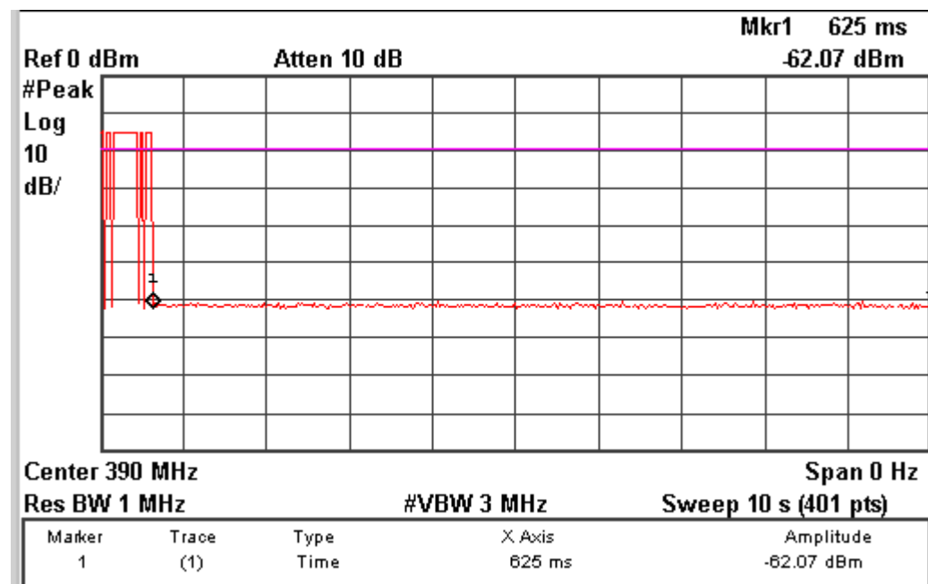
Figure 9 Cease Operation Graph for 390MHz A code
