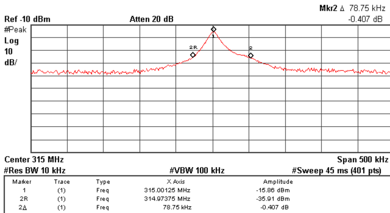
Figure 1 – 20dB Bandwidth Graph for 315MHz D code
