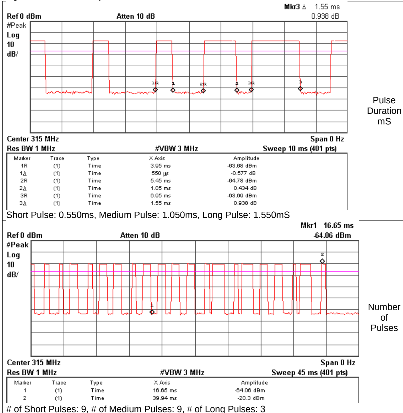
Figure 10 Pulse Train Graphs for 315MHz D code
