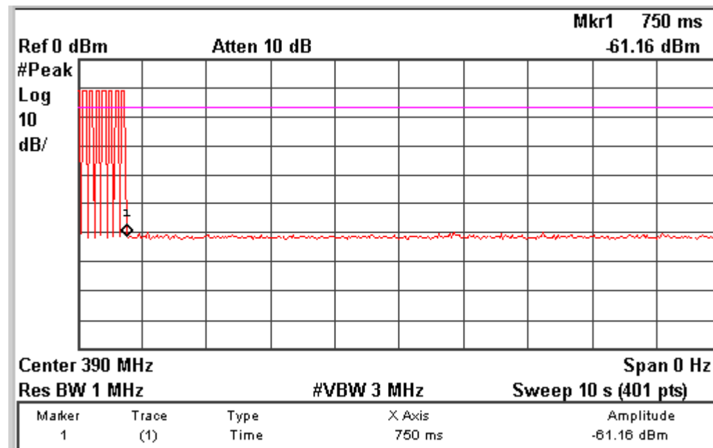
Figure 8 Cease Operation Graph for 390MHz D code
