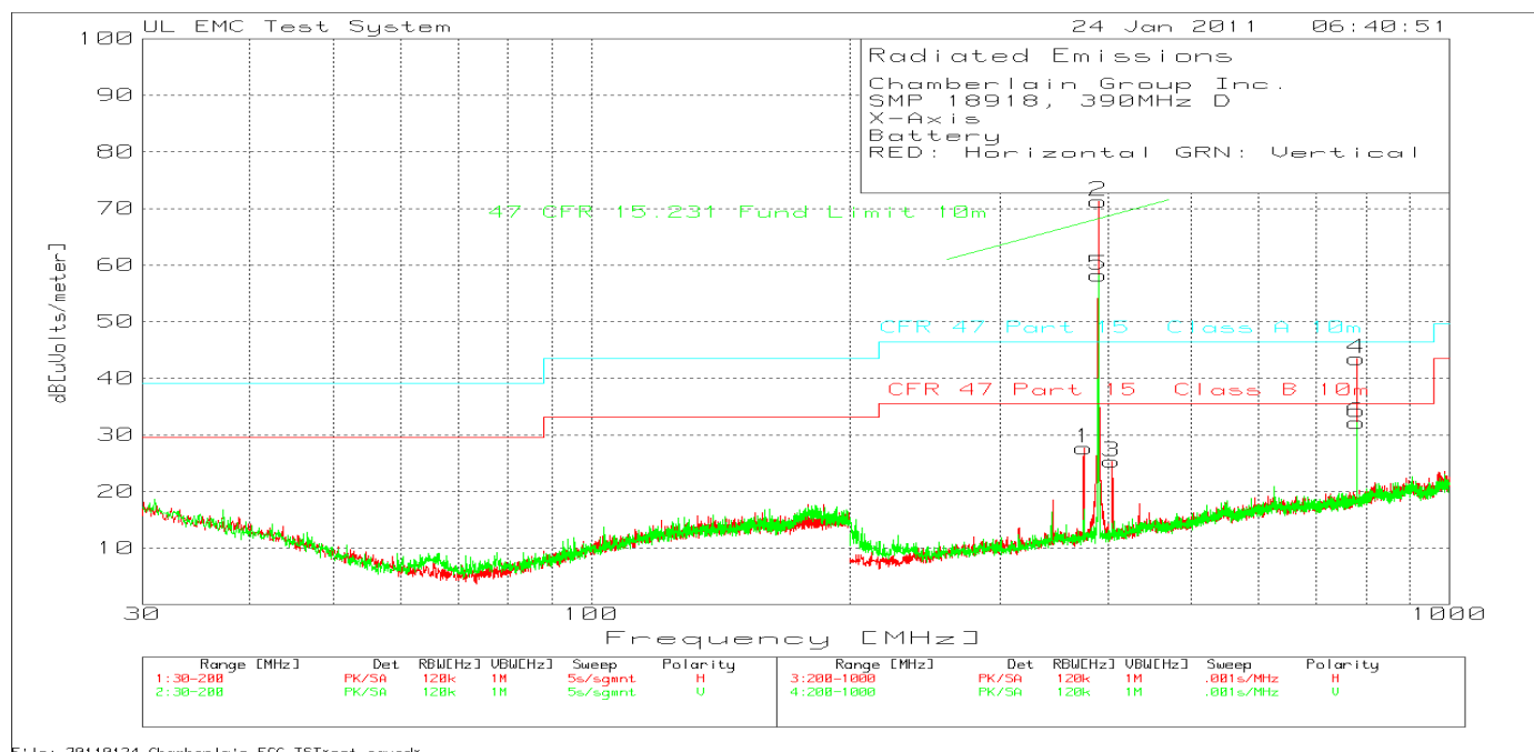
Figure 14 Radiated Emissions Graphs for 390MHz D code
