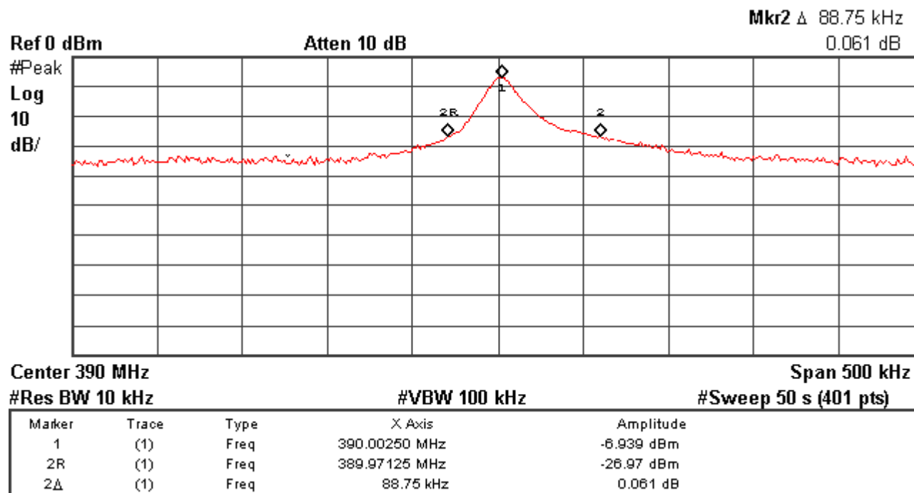
Figure 2 – 20dB Bandwidth Graph for 390MHz D code
