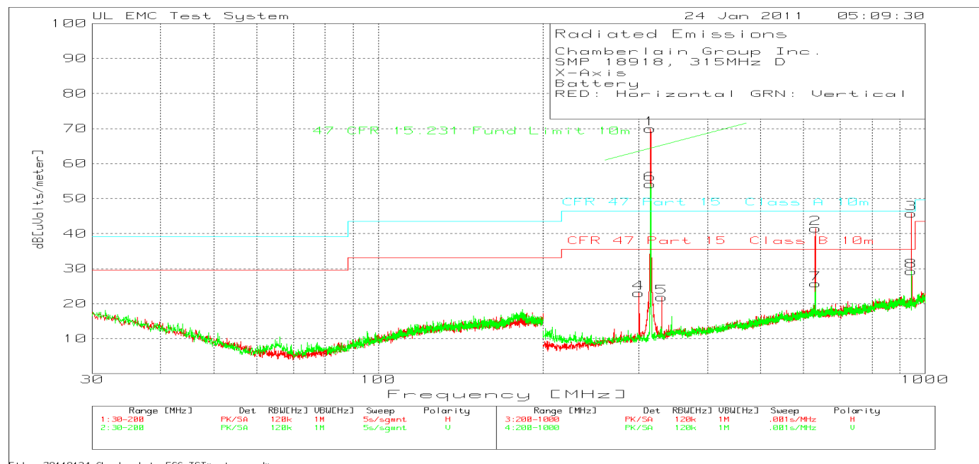
Figure 13 Radiated Emissions Graphs for 315MHz D code
