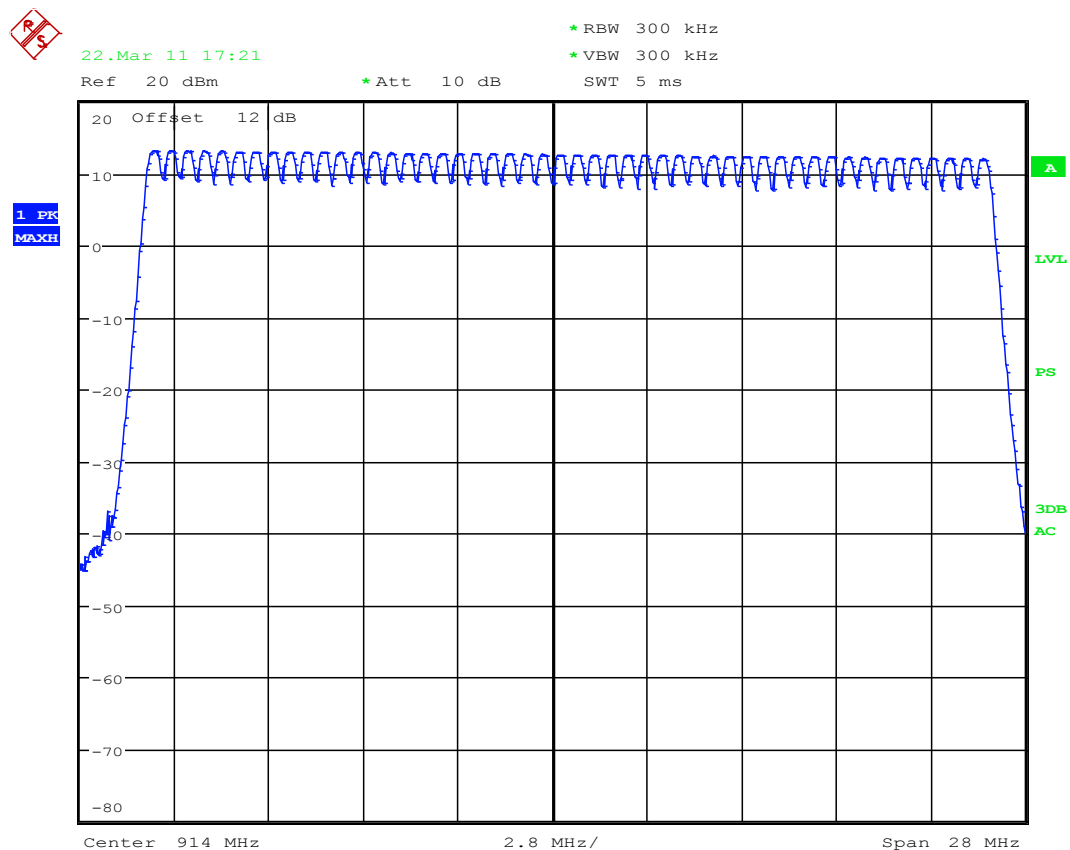
Figure 25 Number of Hopping Frequencies Graphs
