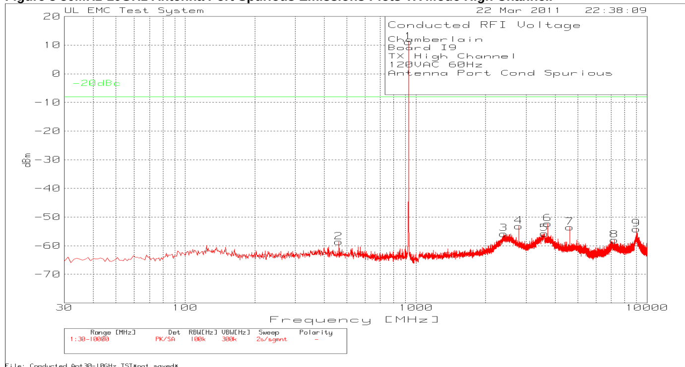
Figure 3 30MHz-10GHz Antenna Port Spurious Emissions Plots TX Mode High Channel.
