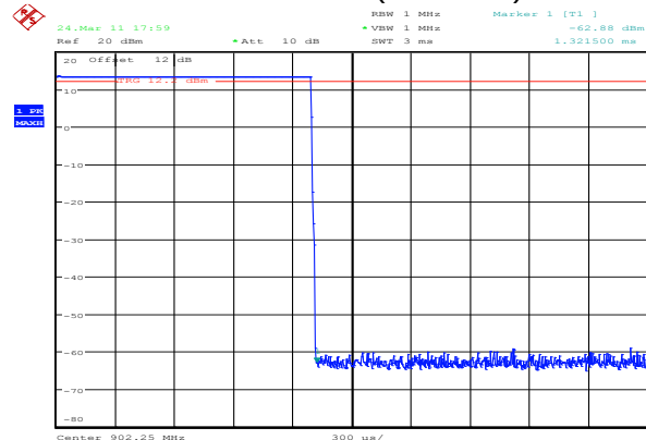
Figure 24 Dwell Time Graphs
