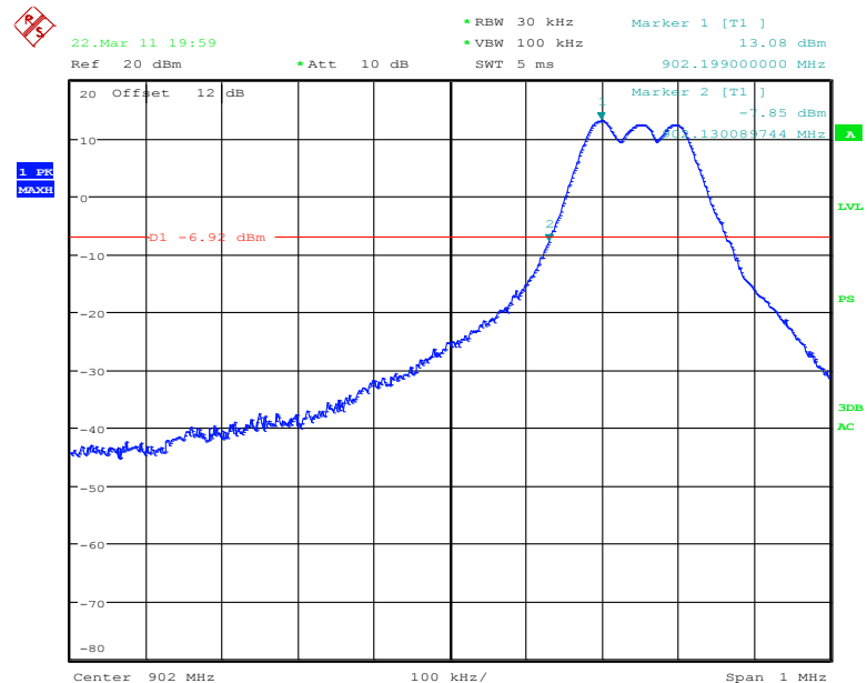
Figure 22 Conducted Band Edge Compliance Graph
