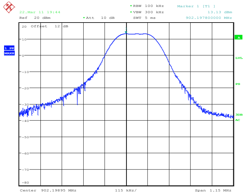
Figure 23 Maximum Peak Output Power Graph
