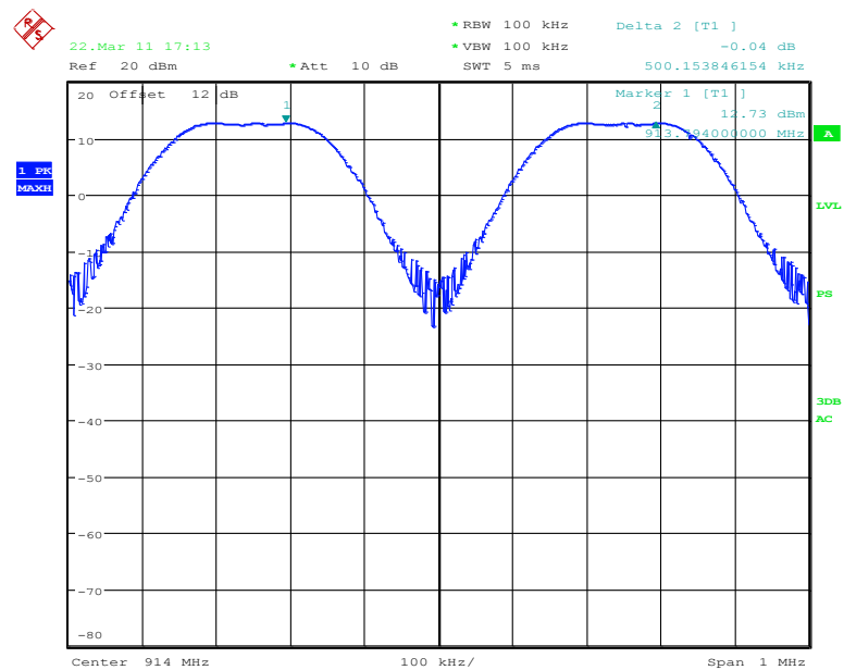
Figure 27 Carrier Frequency Separation Graphs
