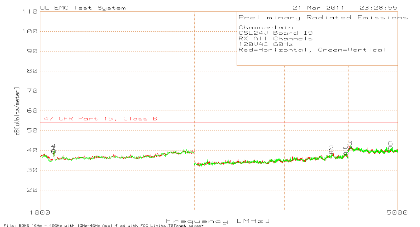
Figure 33 Radiated Emissions above 1GHz, RX Mode, CSL24V
