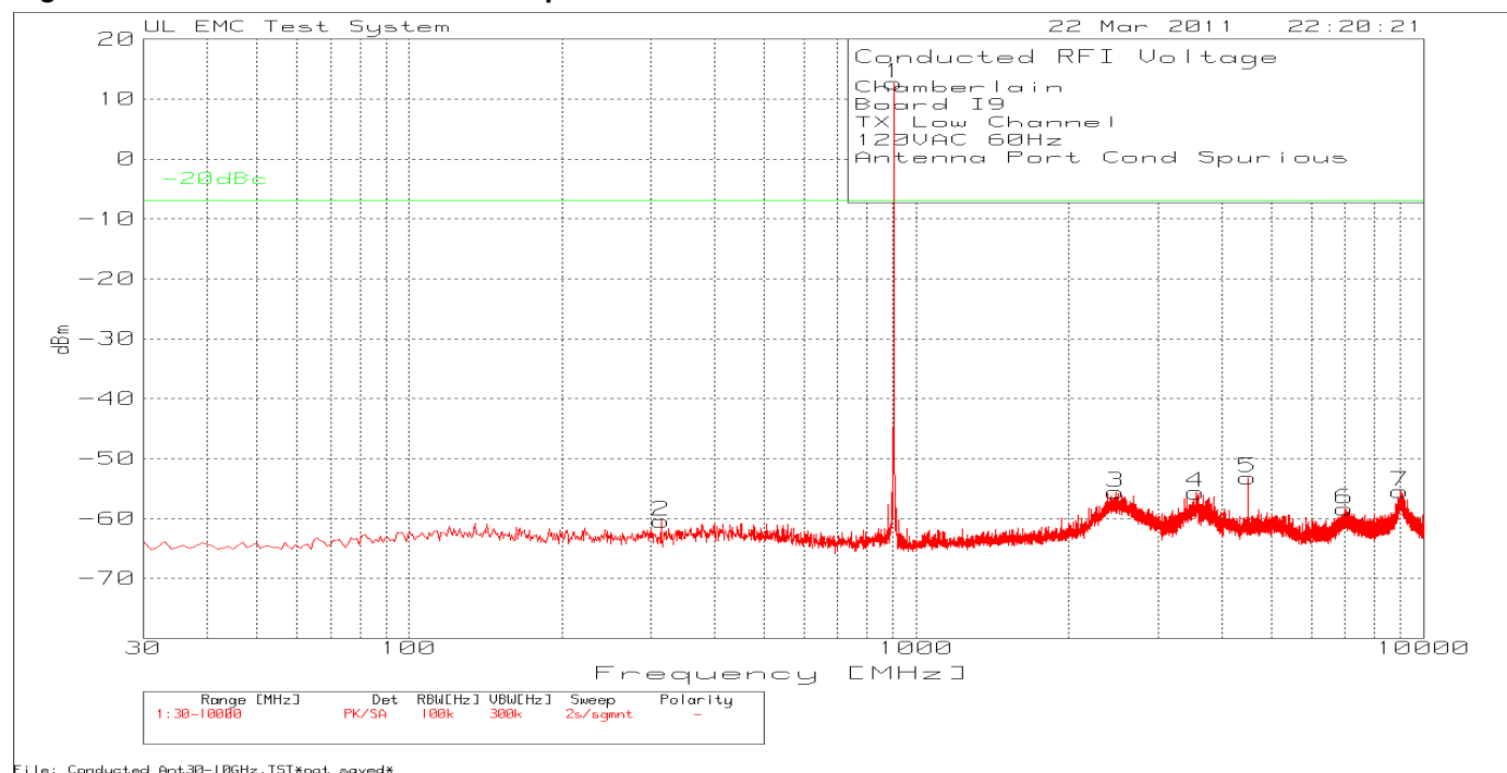
Figure 1 30MHz-10GHz Antenna Port Spurious Emissions Plots TX Mode Low Channel.
