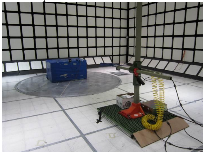
Near Field Measurements Setup
