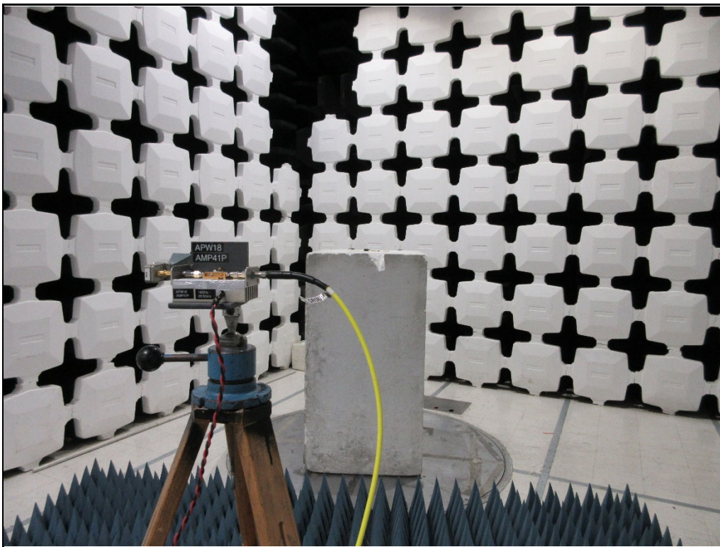
Test Setup for Spurious Radiated Emissions, Above 18GHz – Antenna Polarization Horizontal
