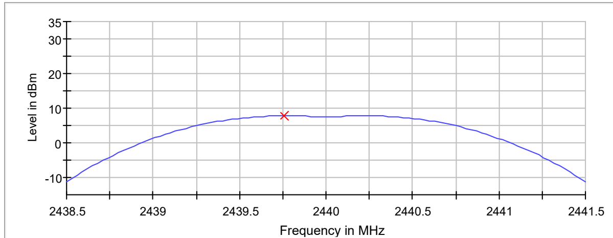
Peak Power
