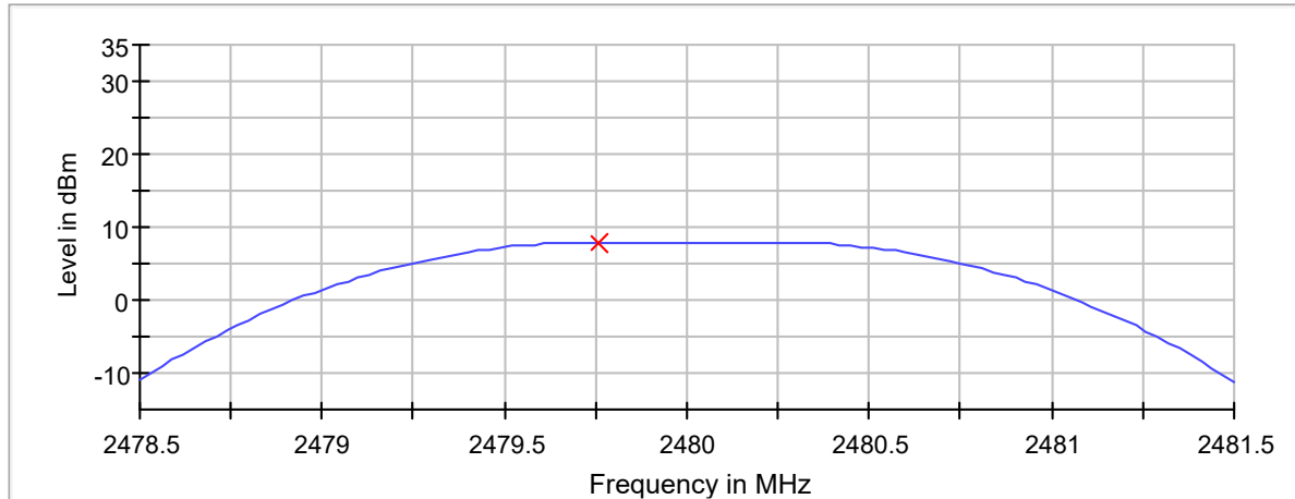
Peak Power
