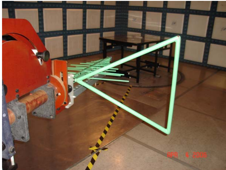
Test Set-up for Radiated Emissions Horizontal Polarization
