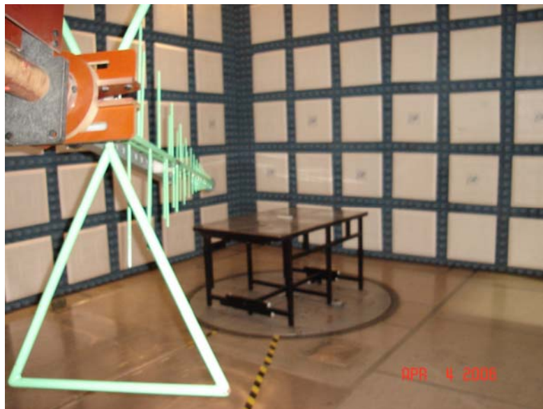
Test Set-up for Radiated Emissions Vertical Polarization
