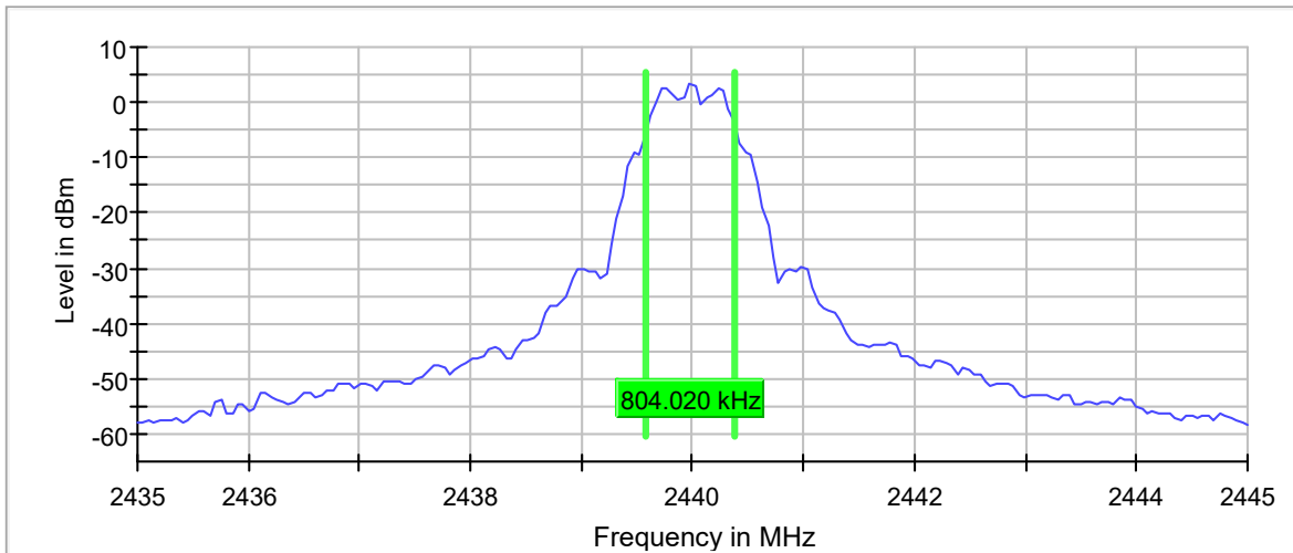
6 dB Bandwidth
