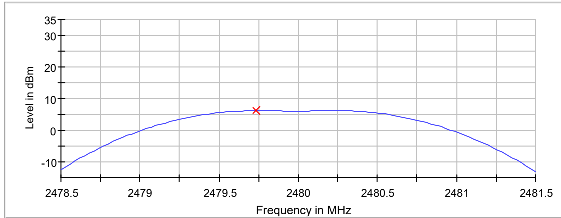
Peak Power
