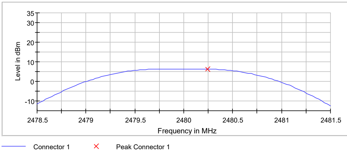
Peak Power
