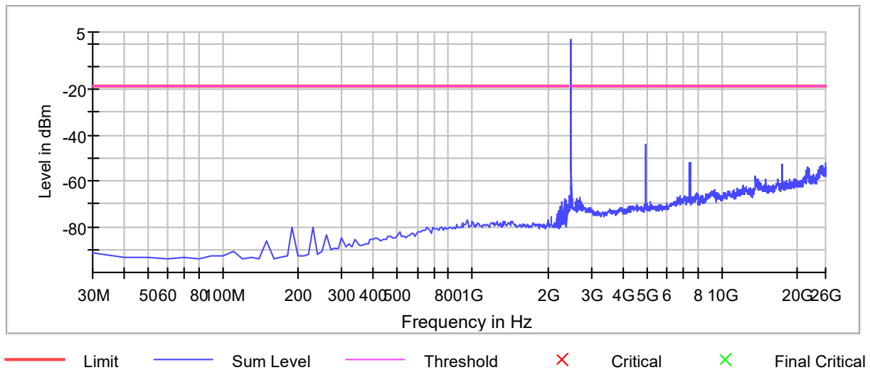
Spurious
