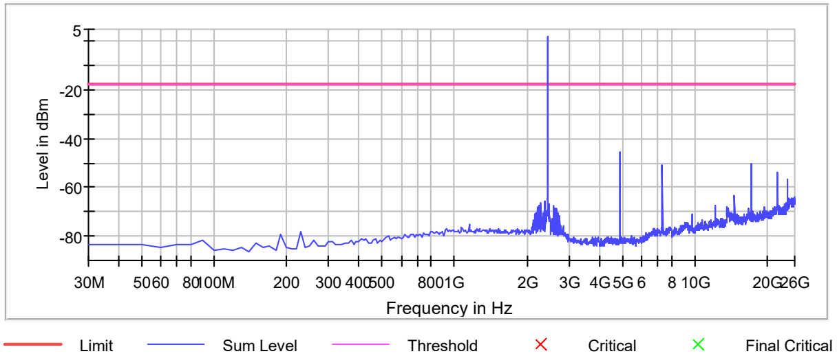
Spurious
