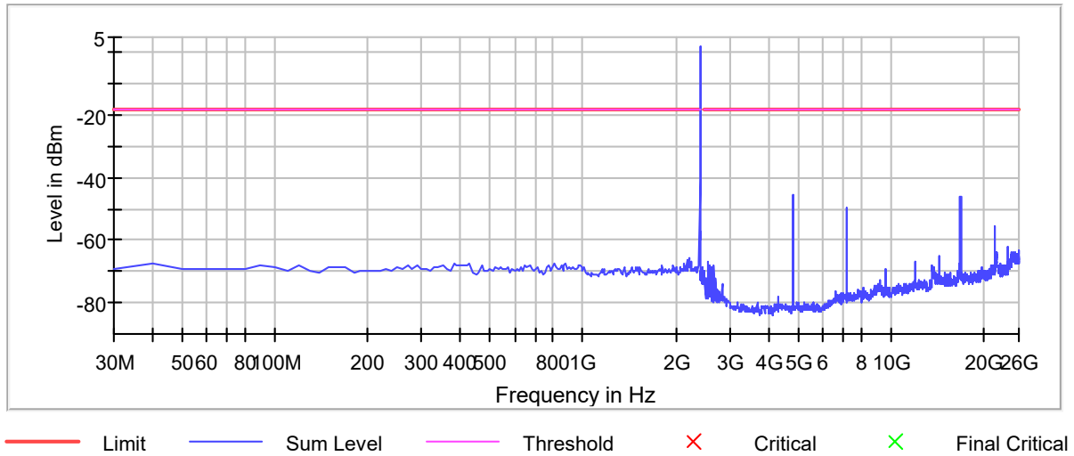
Spurious
