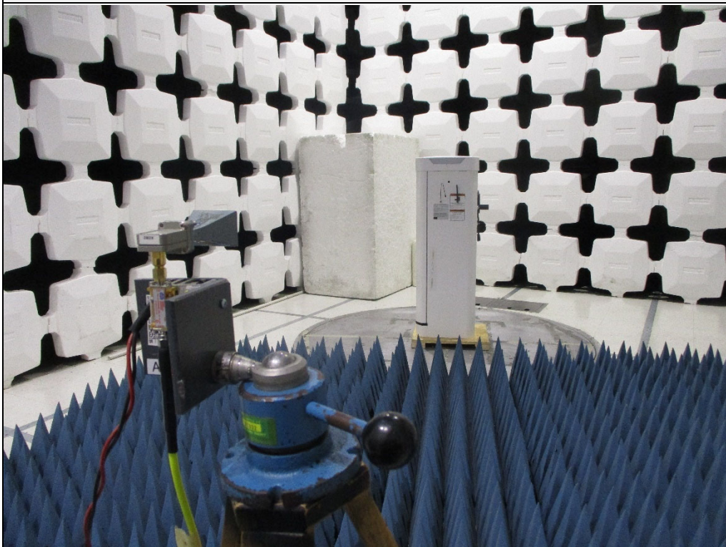
Test Setup for Spurious Emissions: 18GHz to 25GHz, Vertical Polarization
