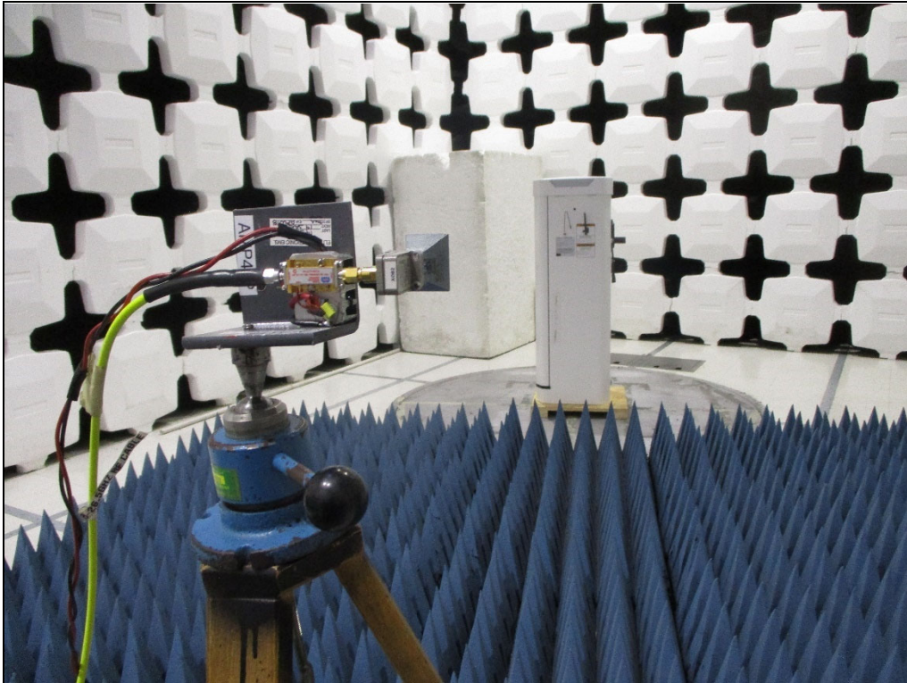
Test Setup for Spurious Emissions: 18GHz to 25GHz, Horizontal Polarization
