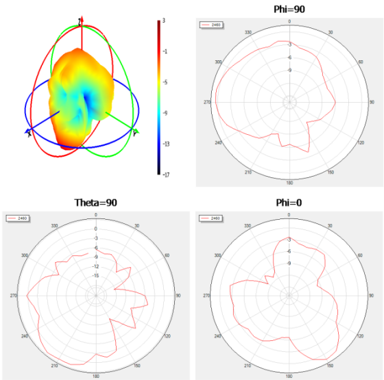
方向辐射图Radiation Patterns
