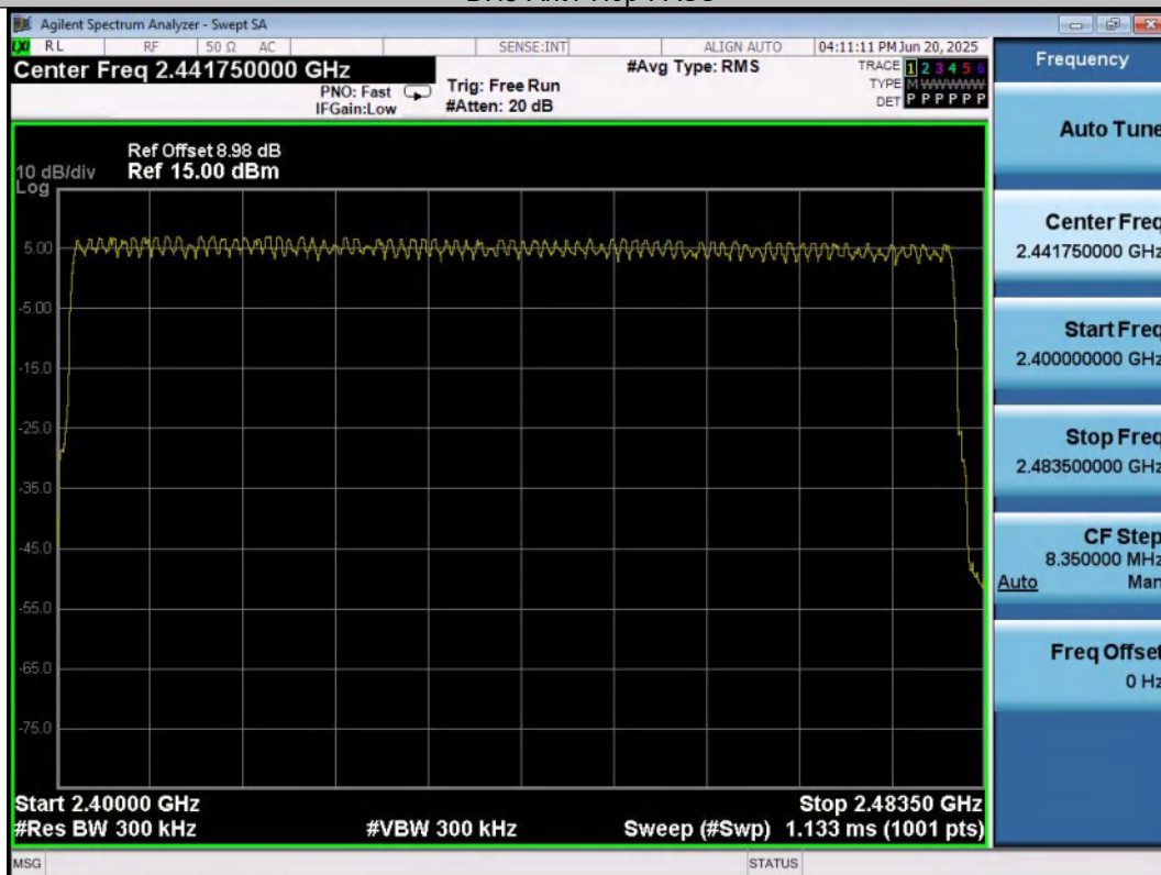
2DH5-Ant1-Hop-PASS
