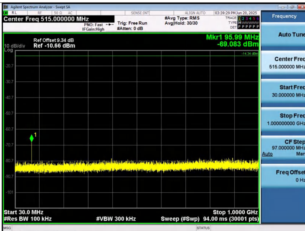
DH5-Ant1-2480-30~1000-PASS
