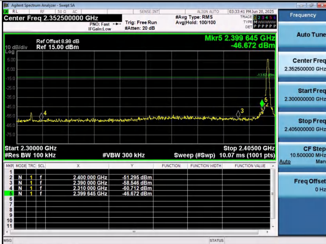
DH5-Ant1-2402-PASS
