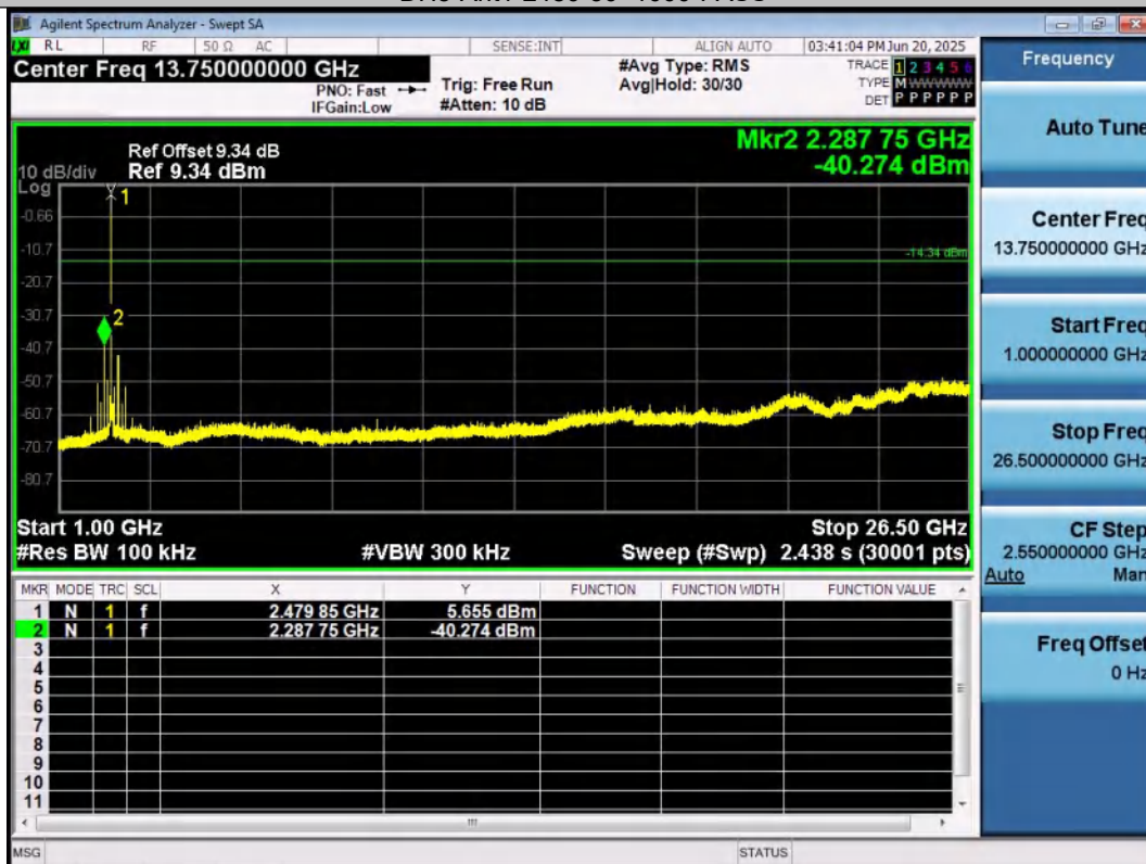
DH5-Ant1-2480-1000~26500-PASS
