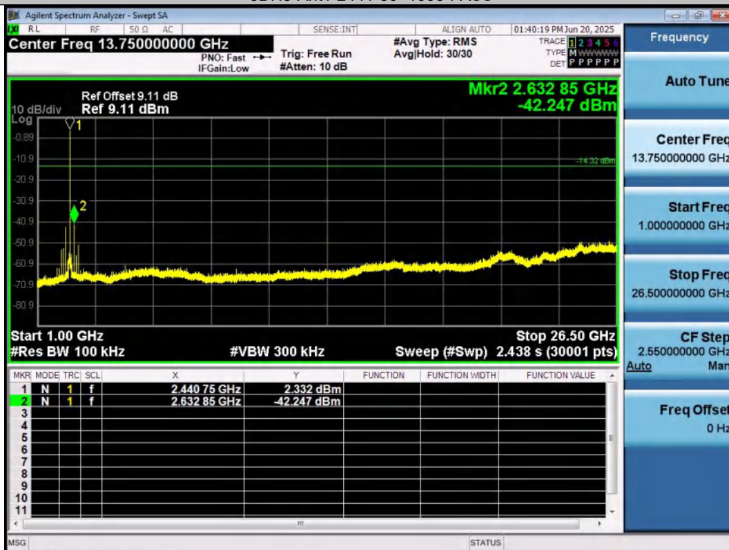
3DH5-Ant1-2441-1000~26500-PASS
