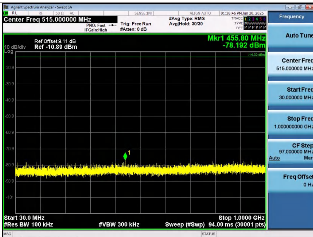
3DH5-Ant1-2441-30~1000-PASS
