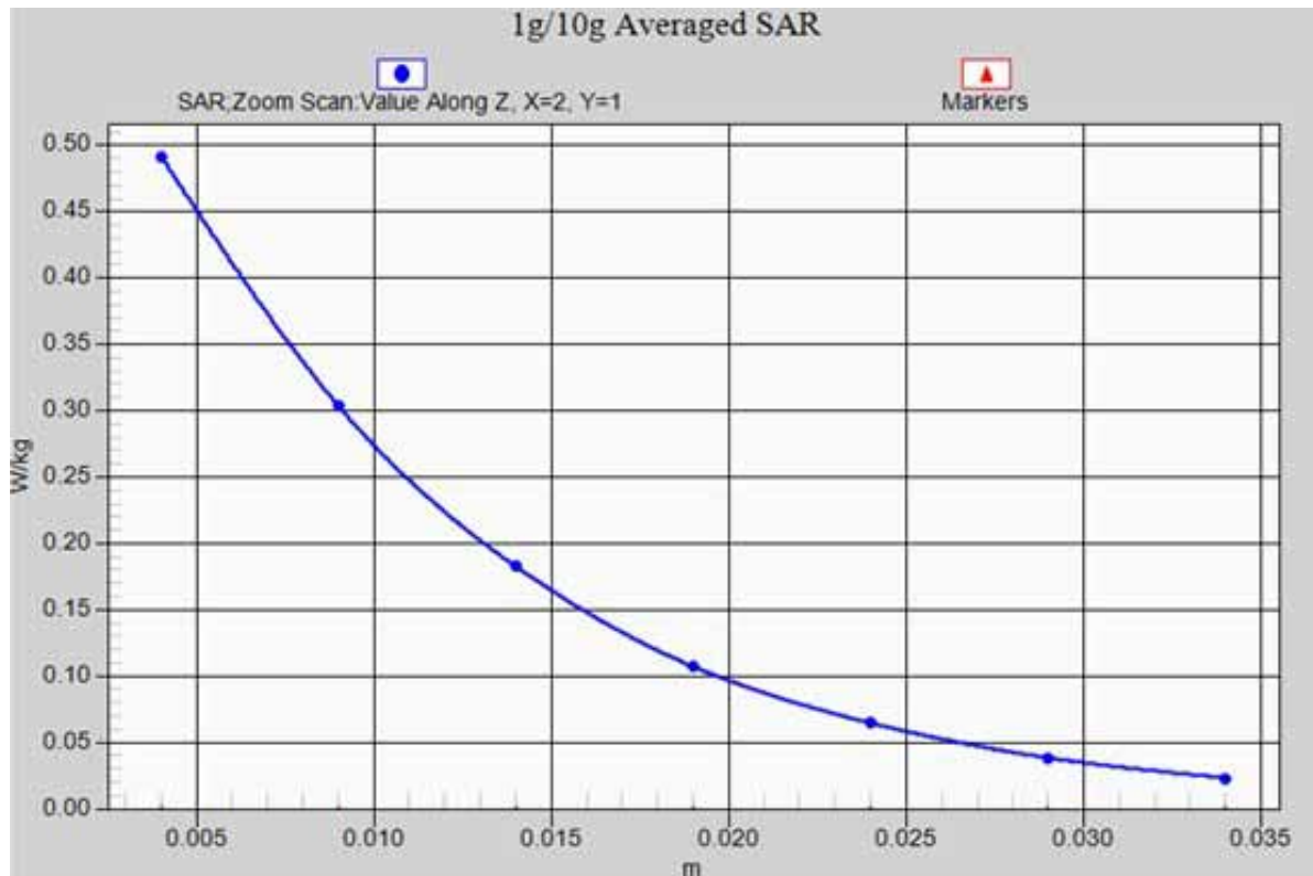
PCS1900 LEFT/TILT-Mid_ z-axis scan
