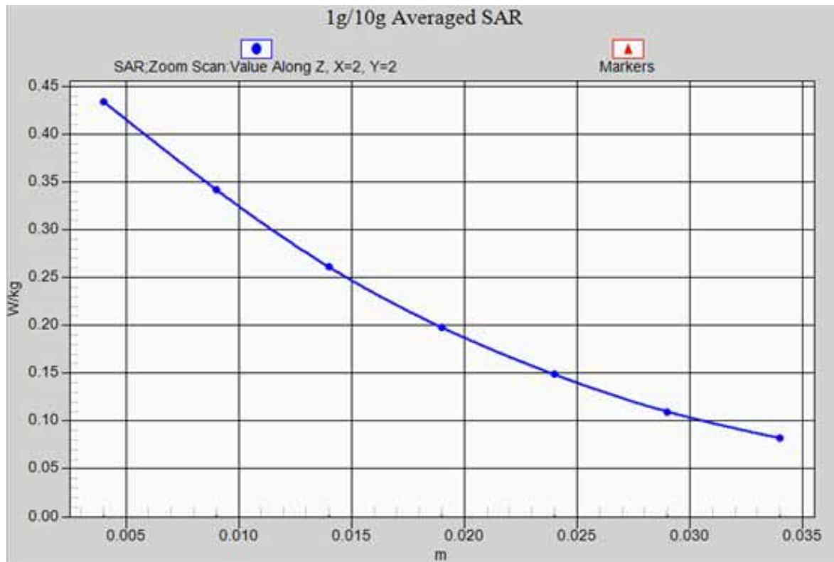
GSM850 RIGHT/CHEEK-High_ z-axis scan
