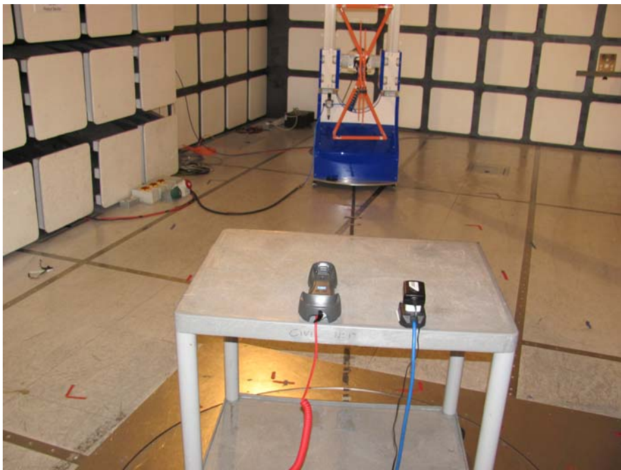
Radiated Emissions
