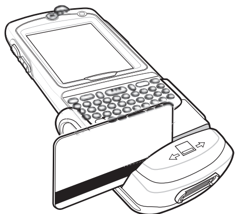
Figure 7-12 Magnetic Stripe Card Swiping
