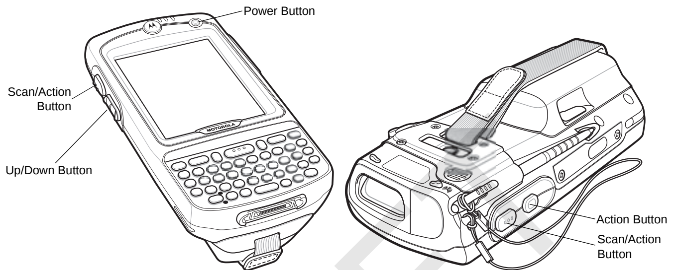
Figure 2-21 Function Buttons
