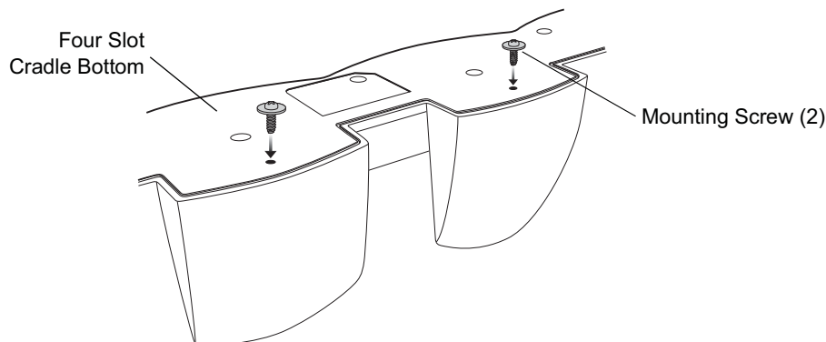
Figure 2-12 Cradle Mounting Screws
