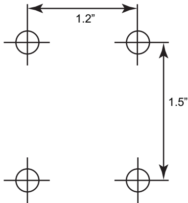
Figure 2-15 Vehicle Cradle Mounting Template
