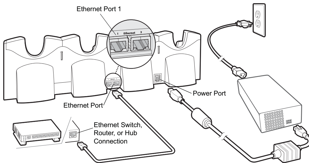
Figure 2-4 Four Slot Ethernet Cradle Connection
