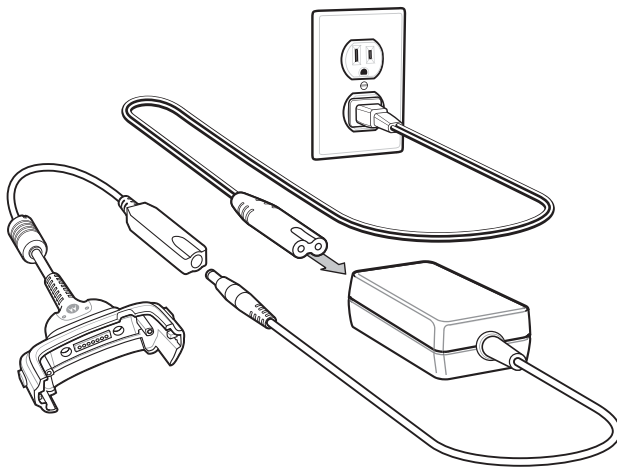
Figure 2-21 Charge Only Cable
