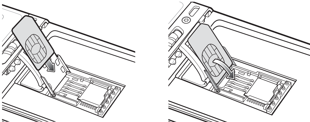
Figure 1-4 Inserting the SIM Card
