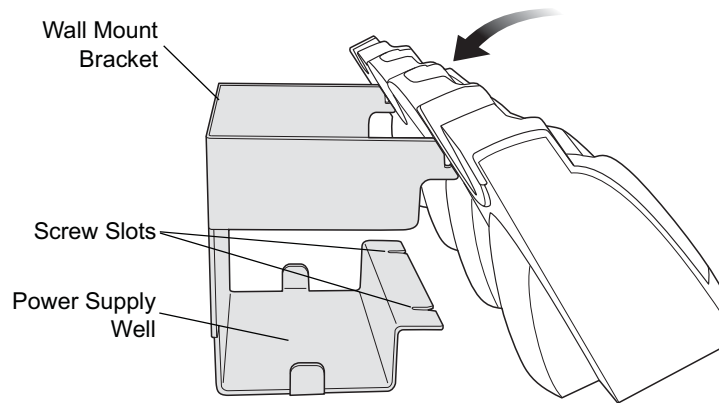
Figure 2-13 Wall Mount Bracket
