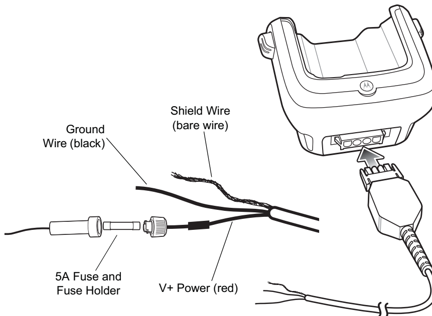
Figure 2-16 Vehicle Cradle Power Connection
