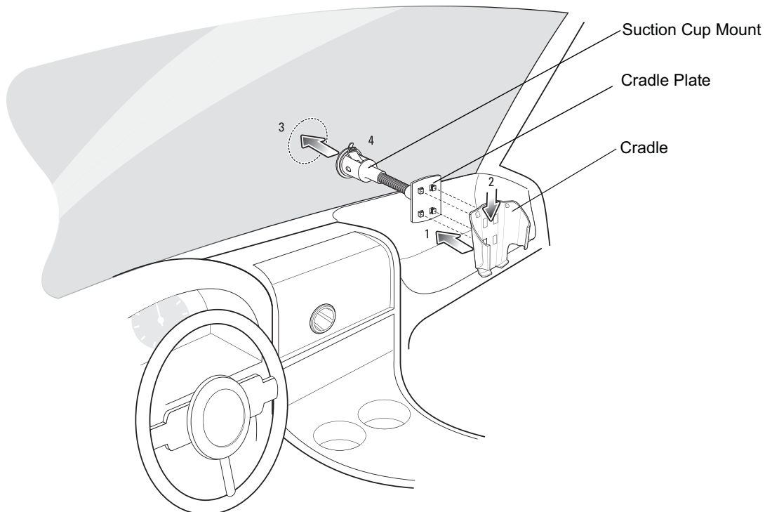
Figure 2-25 Windshield Installation
