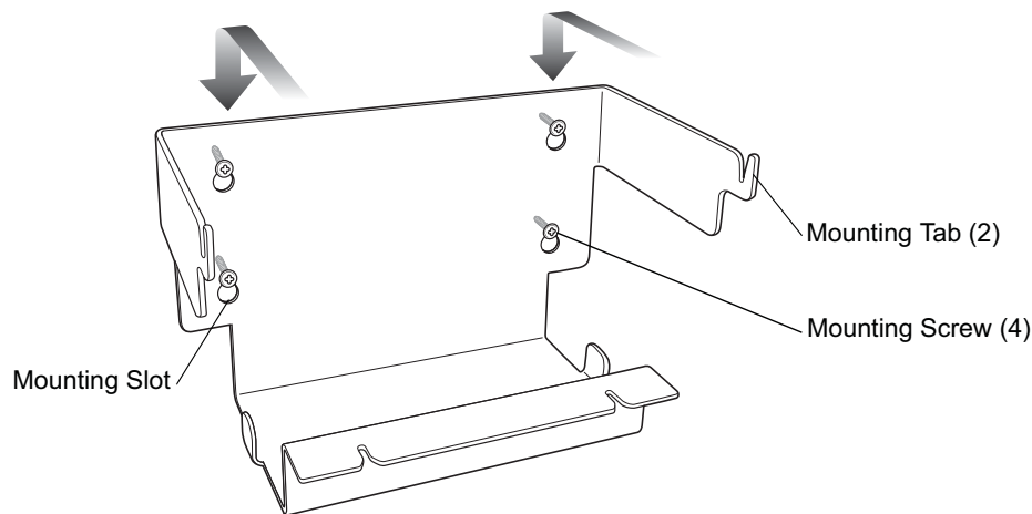
Figure 2-11 Wall Mount Bracket
