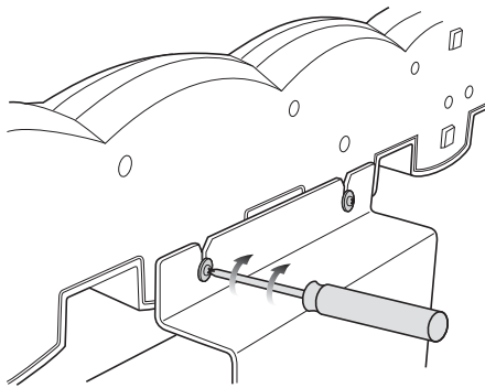
Figure 2-14 Mounting Screws
