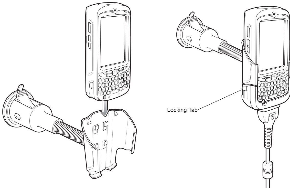
Figure 2-26 Insert MC55 into Vehicle Holder
