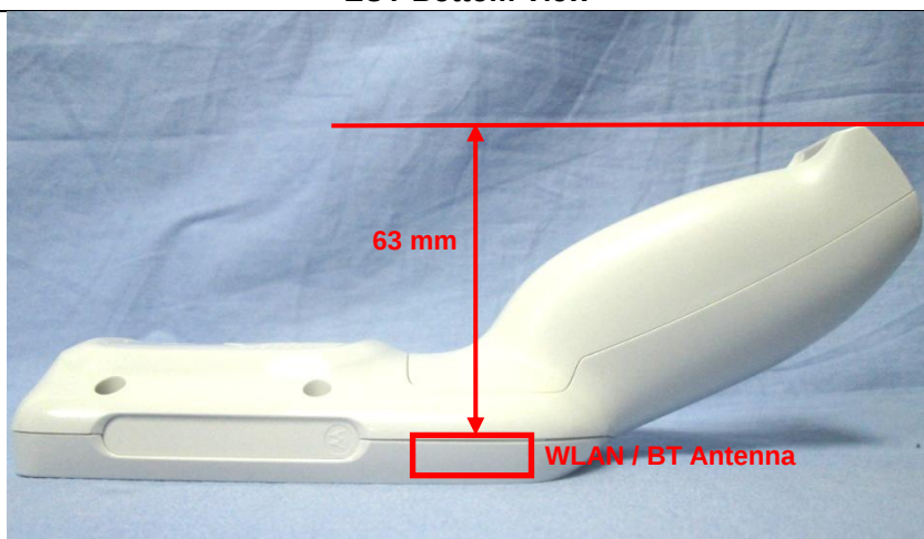
EUT Side View
