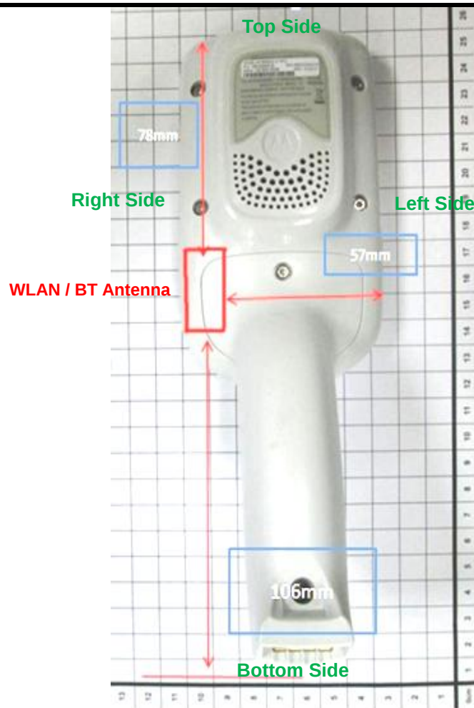
EUT Bottom View
