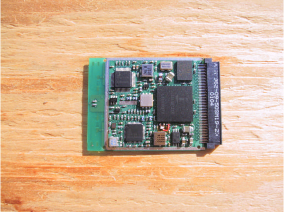
Socket 802.11B PCB – Top View
