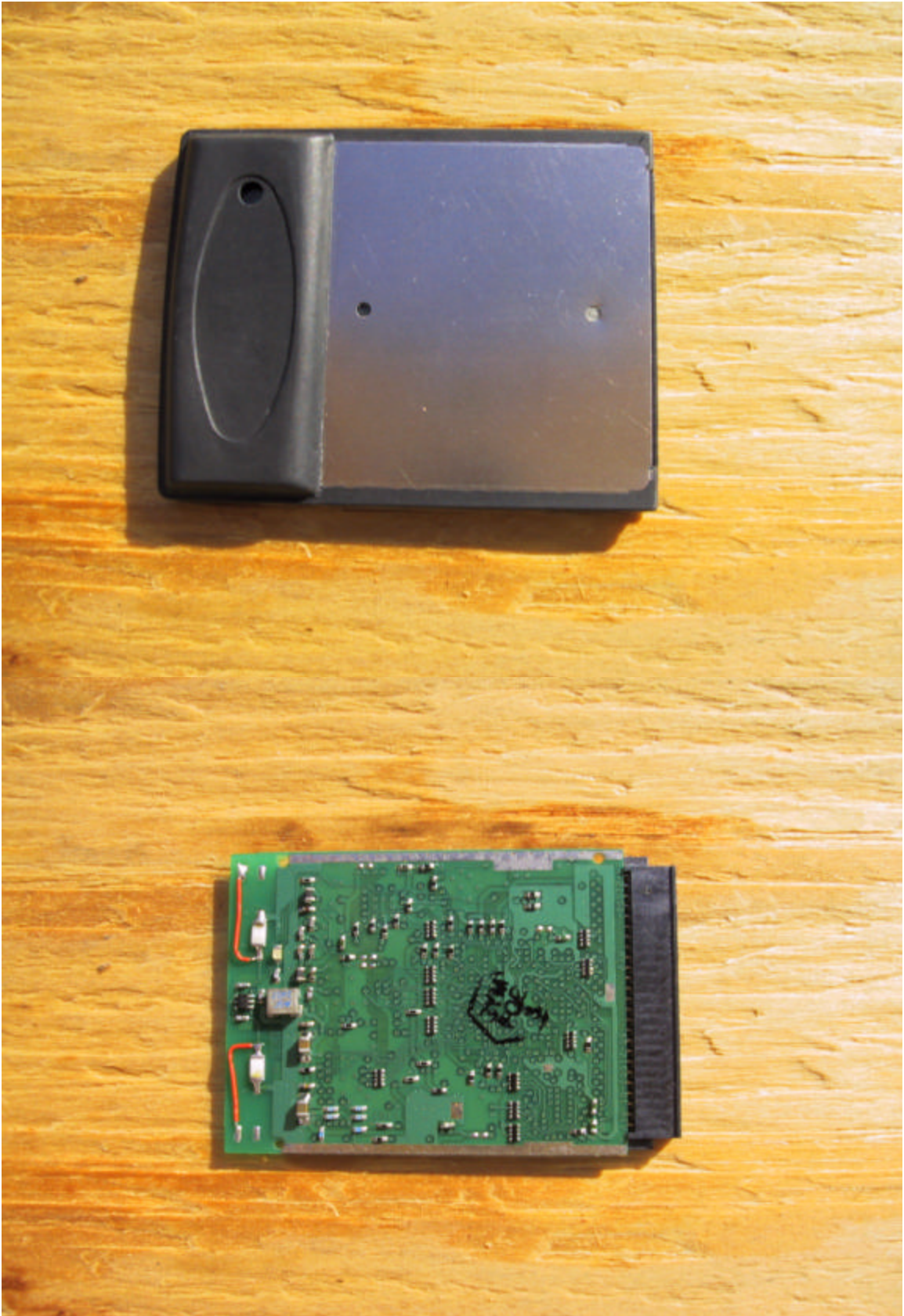
Socket 802.11B – Enclosure Top View / PCB Bottom View
