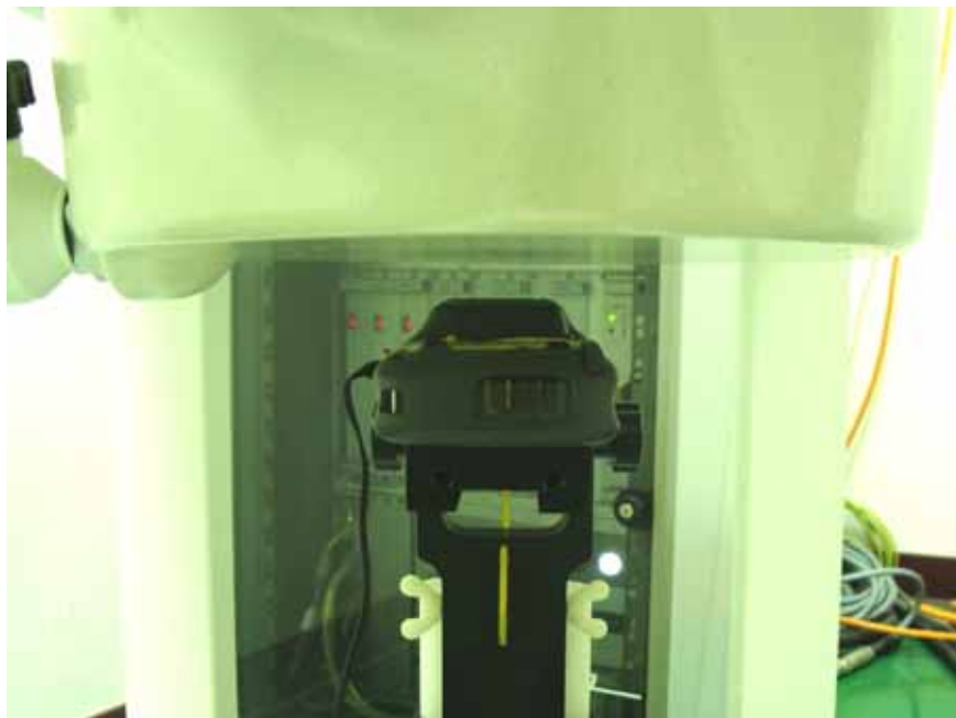
Bottom of the DUT with Battery 2 - with Phantom 1.5 cm Gap
