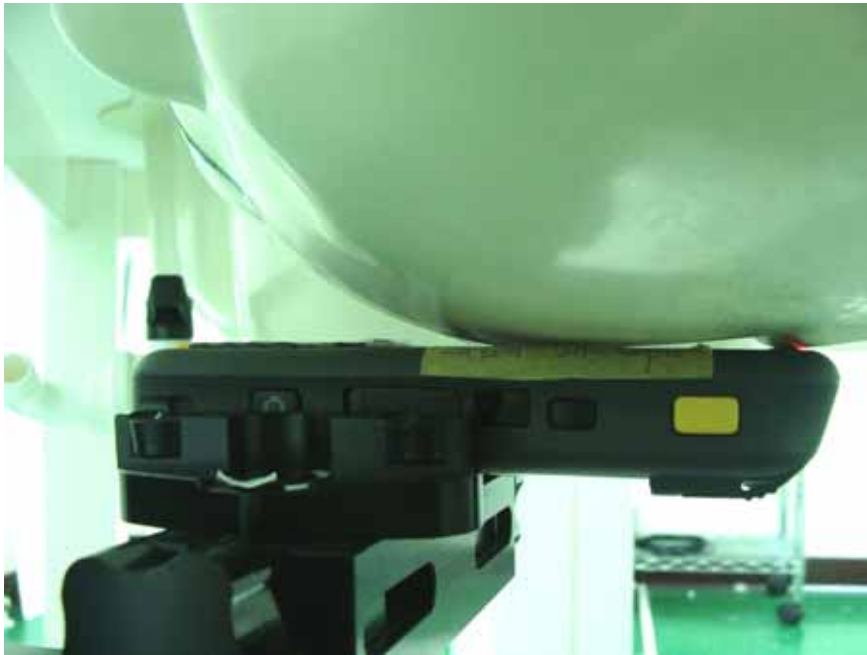
DUT with Battery 1 - Left Cheek
