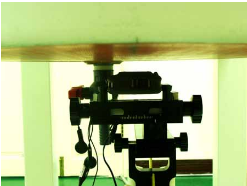
Bottom of the DUT with Battery 1 - with Phantom 1.5 cm Gap
