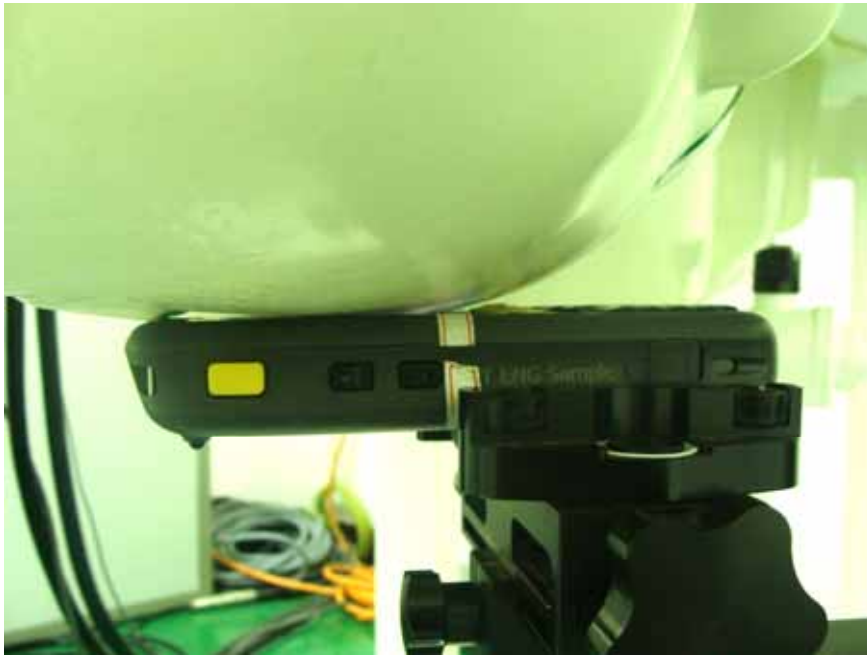
DUT with Battery 2 - Right Cheek
