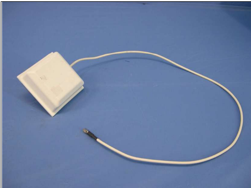
Antenna: ML-5299-WPNA1-01
