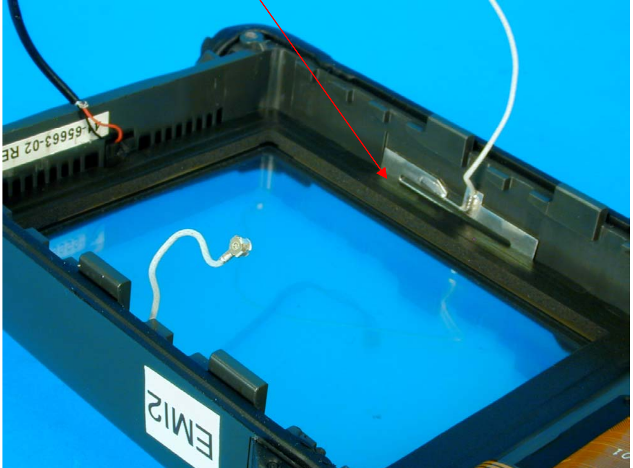
Antenna View 1
