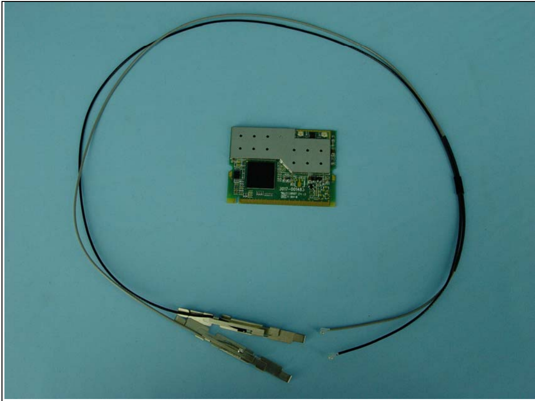
Antenna 2
