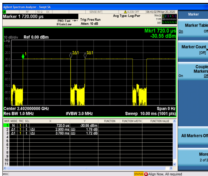
Time-domain plot for Bluetooth transmission signal
