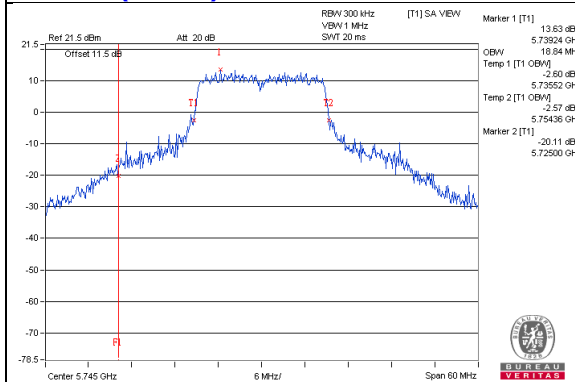
802.11ac(VHT20)_Chain2 / CH149
