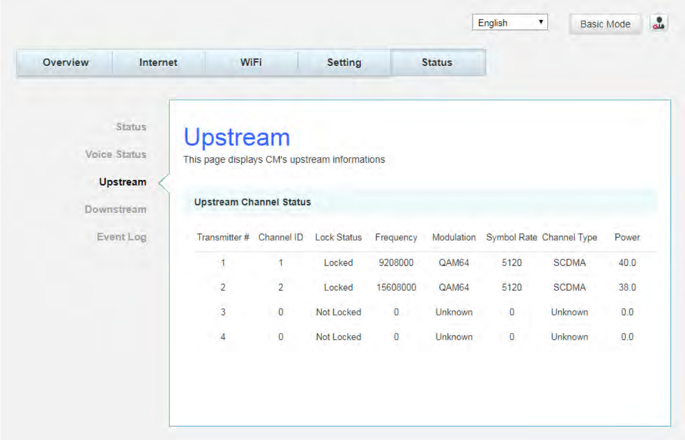
Fig.2-32 Status\Upstream
