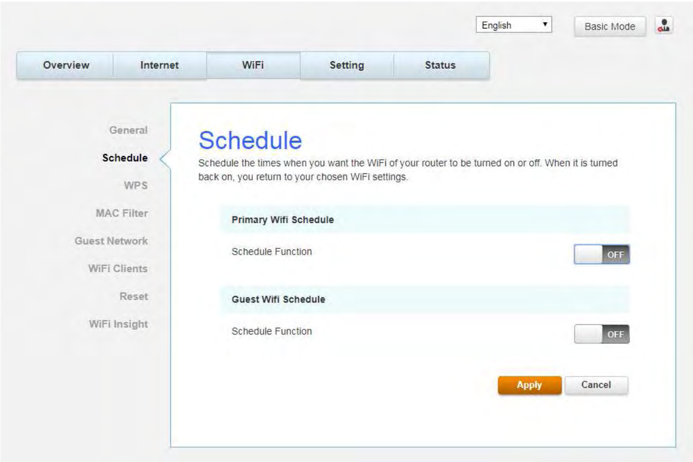
Fig.2-17 Wi-Fi\Schedule
