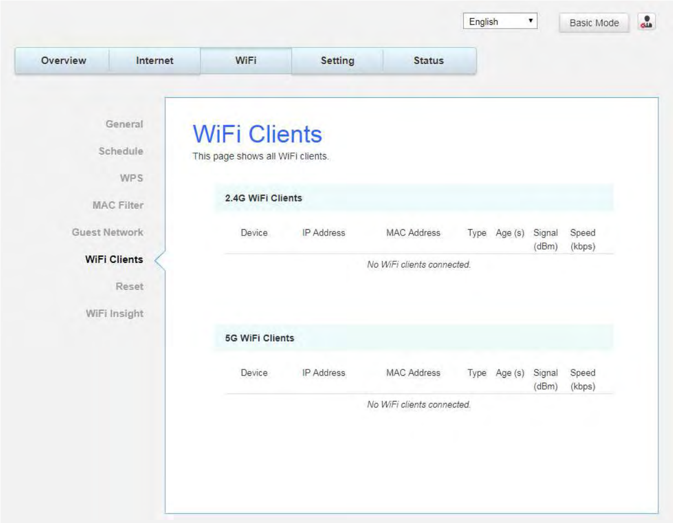
Fig.2-21 Wi-Fi\Wi-Fi Clients
