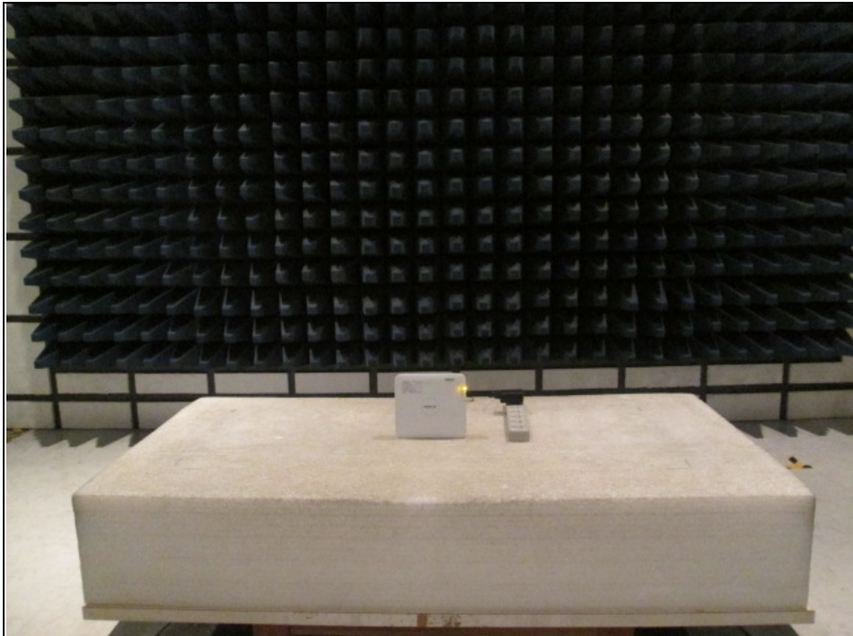
Radiated Emissions below 1 GHz Test
