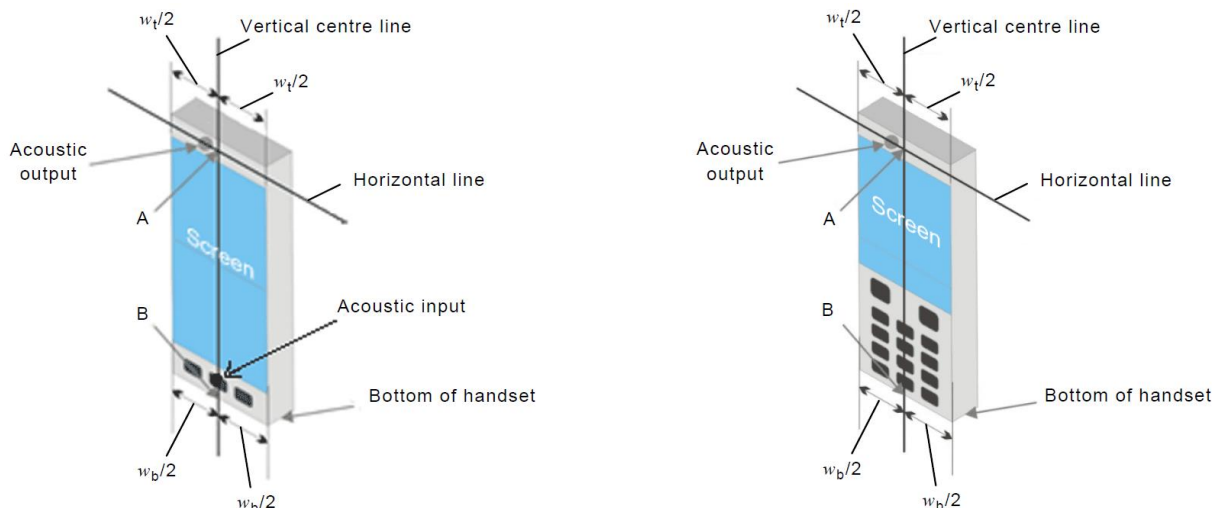
Fig-6.1 Illustration for Handset Vertical and Horizontal Reference Lines
