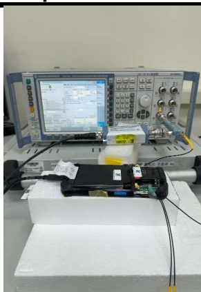
Setup for Conducted Power Test (for WCDMA / LTE Band)
