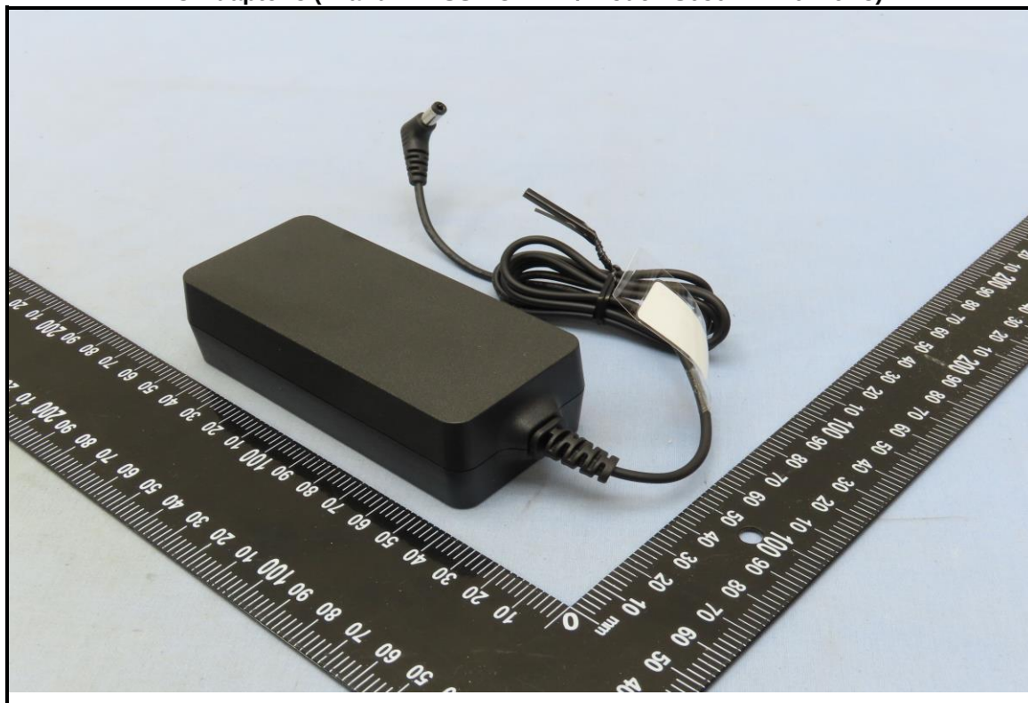
AC Adapter 3 (Brand: MASS POWER / Model: S050-1A120416B3)
