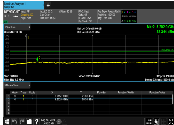
N25(10M)_DFT-s- OFDM_QPSK_Edge_1RB_Left_High_CH
