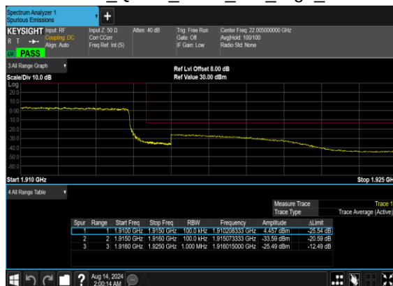
N25(10M)_DFT-s- OFDM_QPSK_Outer_Full_High_CH
