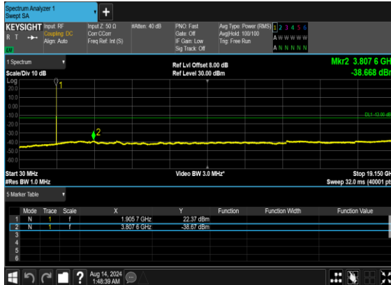
N25(10M)_DFT-s- OFDM_BPSK_Edge_1RB_Left_High_CH
