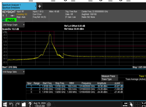
N25(10M)_DFT-s- OFDM_BPSK_Edge_1RB_Right_High_CH
