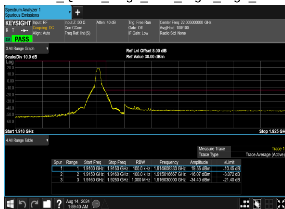
N25(10M)_DFT-s- OFDM_QPSK_Edge_1RB_Right_High_CH
