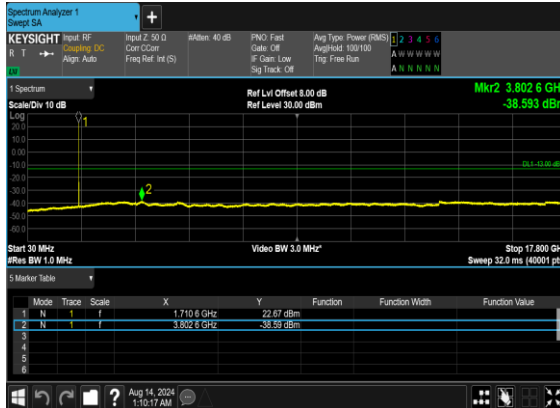
N66(15M)_DFT-s- OFDM_BPSK_Edge_1RB_Left_Low_CH
