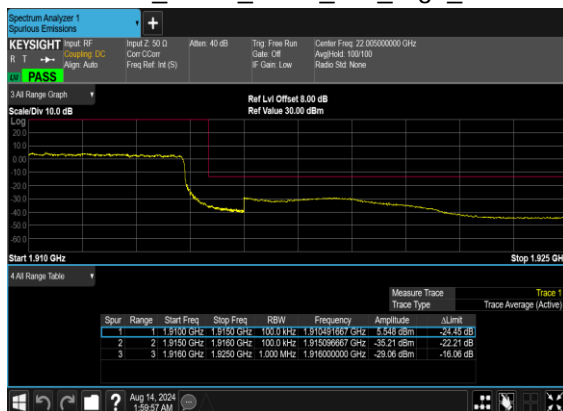
N25(10M)_DFT-s- OFDM_BPSK_Outer_Full_High_CH
