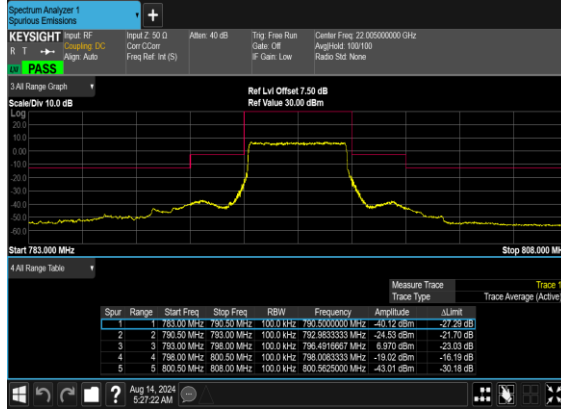
N14(5M)_DFT-s- OFDM_BPSK_Outer_Full_High_CH
