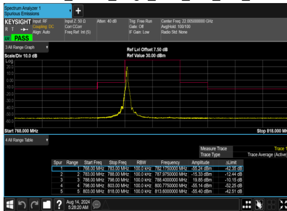
N14(10M)_DFT-s- OFDM_BPSK_Edge_1RB_Left_Mid_CH
