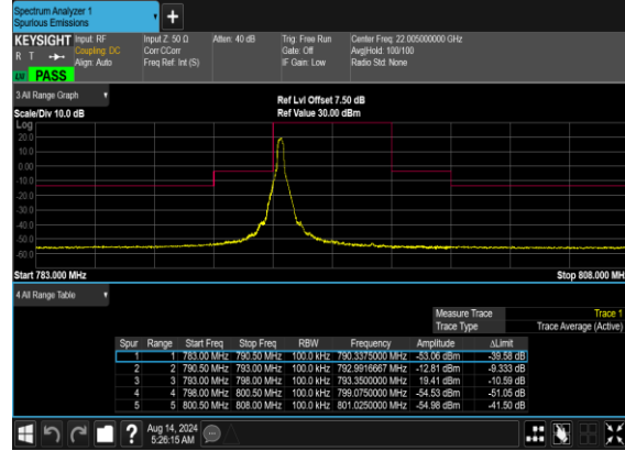
N14(5M)_DFT-s- OFDM_QPSK_Edge_1RB_Left_High_CH
