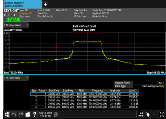
N14(5M)_DFT-s- OFDM_QPSK_Outer_Full_High_CH
