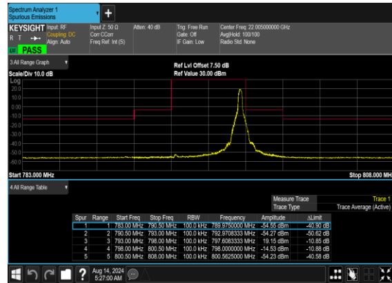
N14(5M)_DFT-s- OFDM_QPSK_Edge_1RB_Right_High_CH
