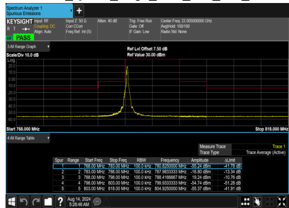
N14(10M)_DFT-s- OFDM_QPSK_Edge_1RB_Left_Mid_CH
