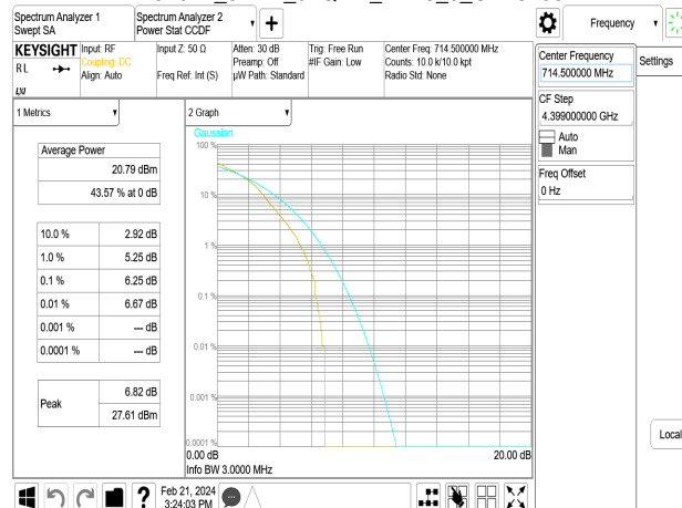
Band12_3MHz_64QAM_RB15_0_CH23165
