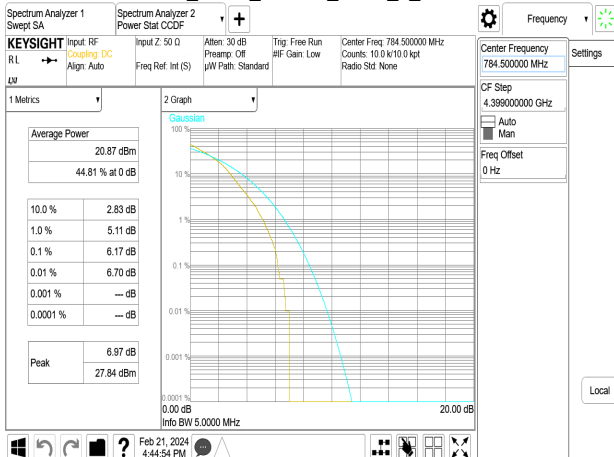
Band13_5MHz_64QAM_RB25_0_CH23255
