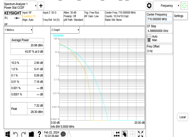
Band17_5MHz_64QAM_RB25_0_CH23790
