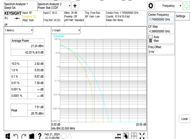
Band4_20MHz_64QAM_RB100_0_CH20300
