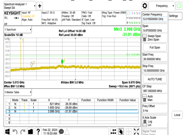
Band26-Part90s_5MHz_QPSK_RB1_0_CH26715
