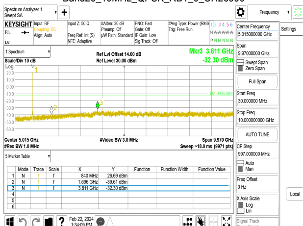
Band26_15MHz_QPSK_RB1_0_CH26865
