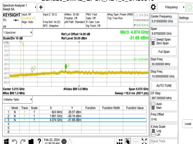
Band26_5MHz_QPSK_RB1_0_CH26815
