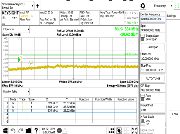
Band26-Part90s_3MHz_QPSK_RB1_0_CH26705
