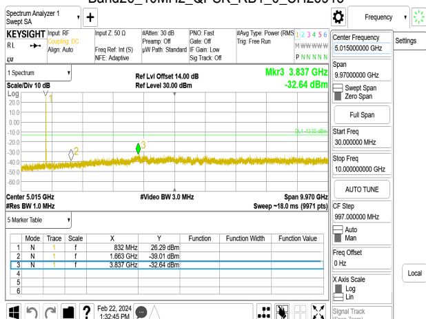
Band26_10MHz_QPSK_RB1_0_CH26990
