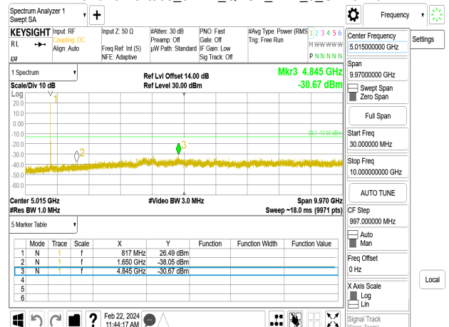
Band26-Part90s_5MHz_QPSK_RB1_0_CH26740
