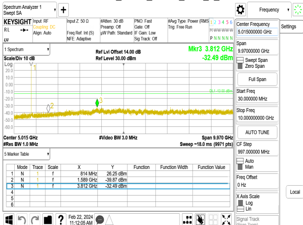
Band26-Part90s_3MHz_QPSK_RB1_0_CH26740
