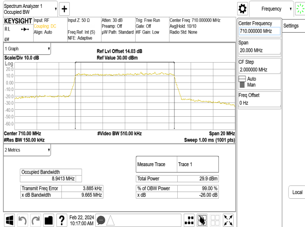
Band17_10MHz_16QAM_RB50_0_CH23800
