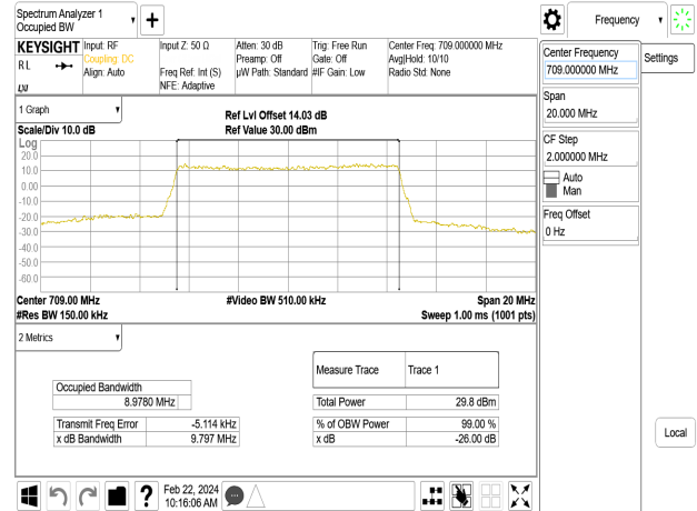
Band17_10MHz_64QAM_RB50_0_CH23790
