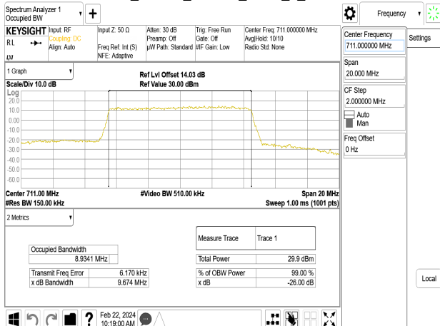
Band17_10MHz_16QAM_RB50_0_CH23800
