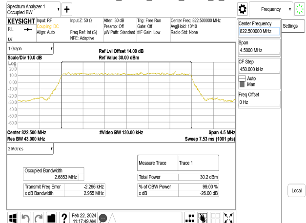
Band26-Part90s_3MHz_QPSK_RB15_0_CH26775
