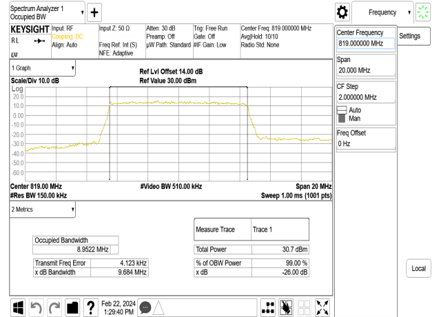
Band26-Part90s_10MHz_16QAM_RB50_0_CH26740
