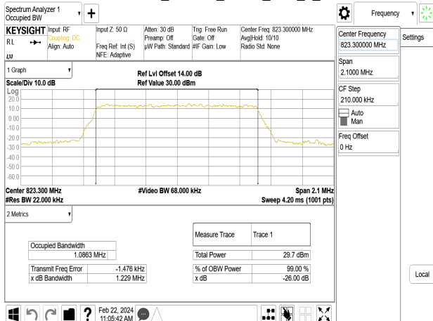
Band26-Part90s_1.4MHz_QPSK_RB6_0_CH26783
