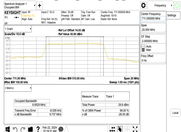
Band17_10MHz_64QAM_RB50_0_CH23800
