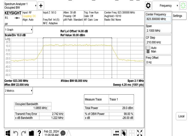
Band26-Part90s_1.4MHz_16QAM_RB6_0_CH26783
