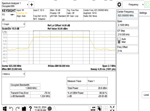
Band26-Part90s_1.4MHz_64QAM_RB6_0_CH26783
