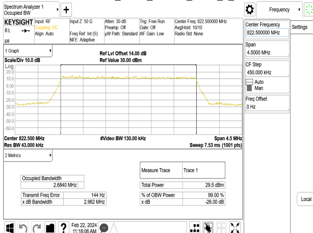
Band26-Part90s_3MHz_16QAM_RB15_0_CH26775
