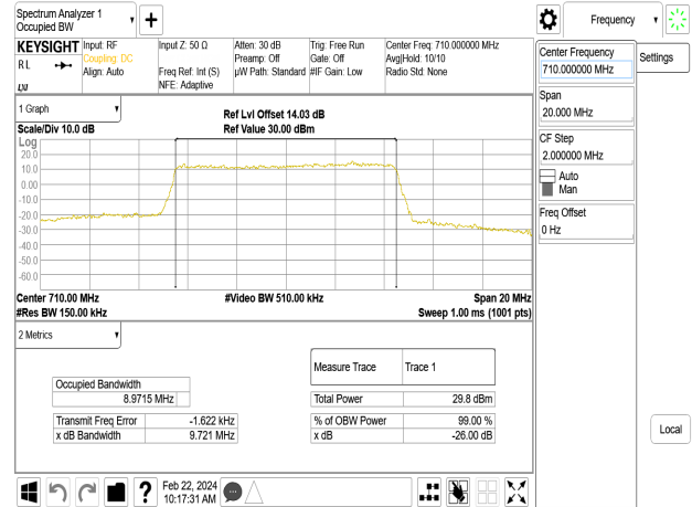
Band17_10MHz_64QAM_RB50_0_CH23800
