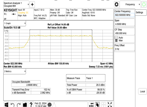
Band26-Part90s_3MHz_64QAM_RB15_0_CH26775
