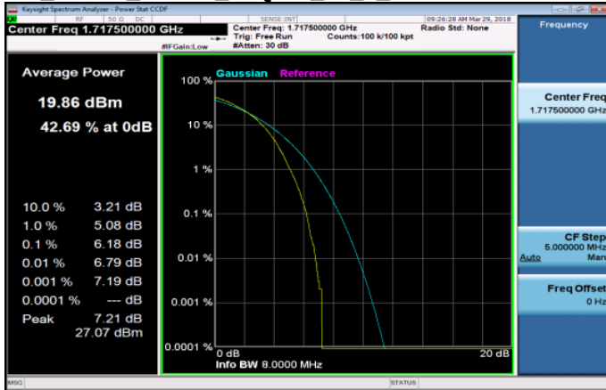
LTE_Band4_15MHz_16QAM_75_0_LowCH20025-1717.5
