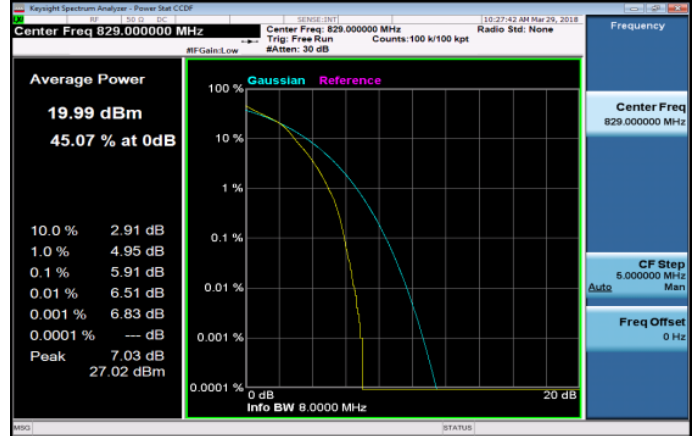
LTE_Band5_10MHz_16QAM_50_0_LowCH20450-829
