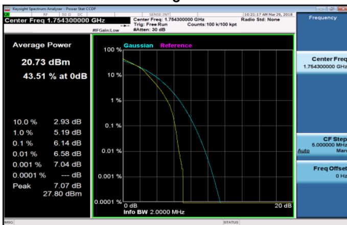
LTE_Band4_1_4MHz_16QAM_6_0_HighCH20393-1754.
