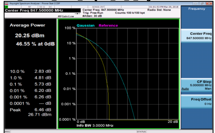
LTE_Band26_3MHz_16QAM_15_0_HighCH27025-847.5
