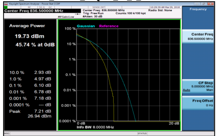
LTE_Band5_10MHz_16QAM_50_0_MidCH20525-836.5
