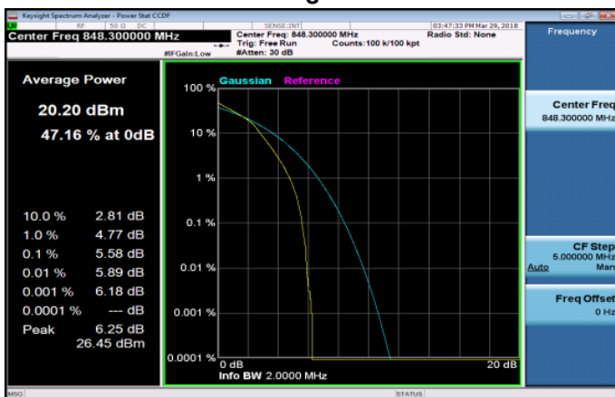
LTE_Band26_1_4MHz_16QAM_6_0_HighCH27033-848.
