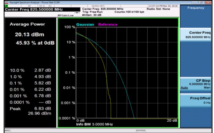
LTE_Band26_3MHz_16QAM_15_0_LowCH26805-825.5
