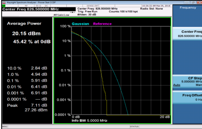
LTE_Band5_5MHz_16QAM_25_0_LowCH20425-826.5
