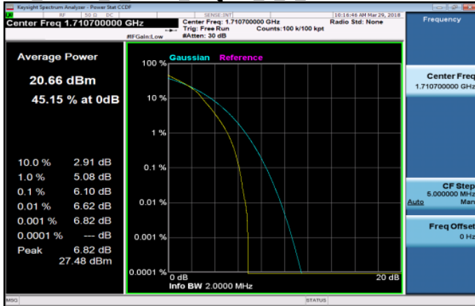
LTE_Band4_1_4MHz_16QAM_6_0_LowCH19957-1710.7
