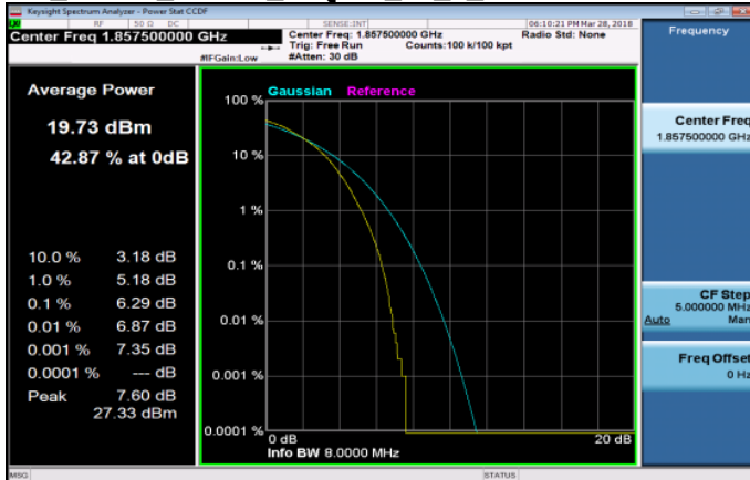
LTE_Band2_15MHz_16QAM_75_0_LowCH18675-1857.5
