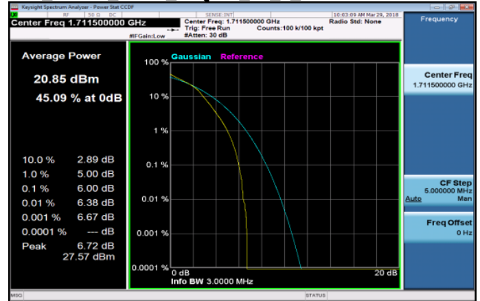
LTE_Band4_3MHz_16QAM_15_0_LowCH19965-1711.5
