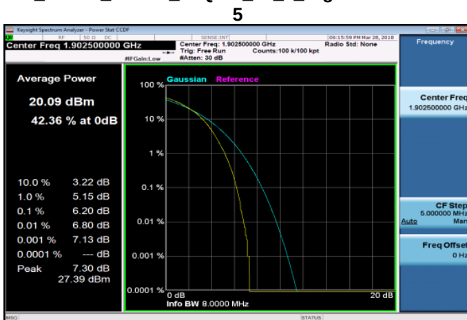
LTE_Band2_15MHz_16QAM_75_0_HighCH19125-1902.
