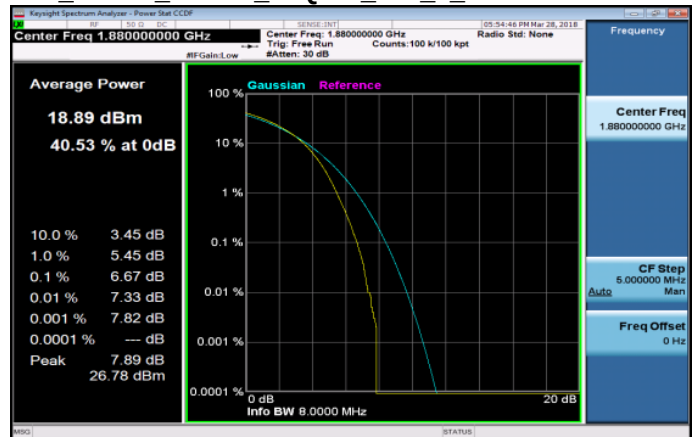
LTE_Band2_20MHz_16QAM_100_0_MidCH18900-1880
