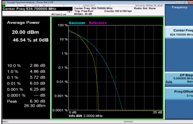
LTE_Band26_1_4MHz_16QAM_6_0_LowCH26797-824.7
