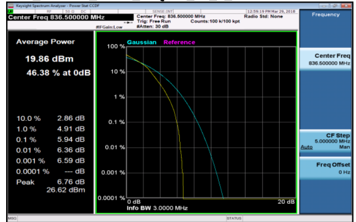
LTE_Band26_3MHz_16QAM_15_0_MidCH26915-836.5
