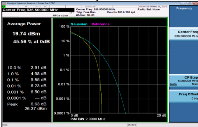
LTE_Band26_1_4MHz_16QAM_6_0_MidCH26915-836.5
