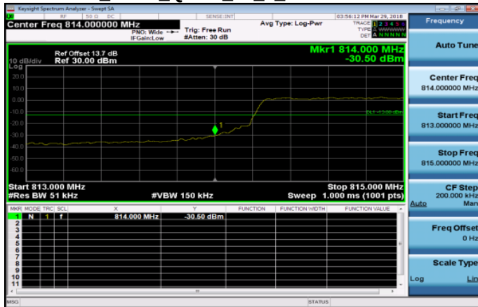
Band26 5MHz_QPSK_25_0_LowCH26715-816.5
