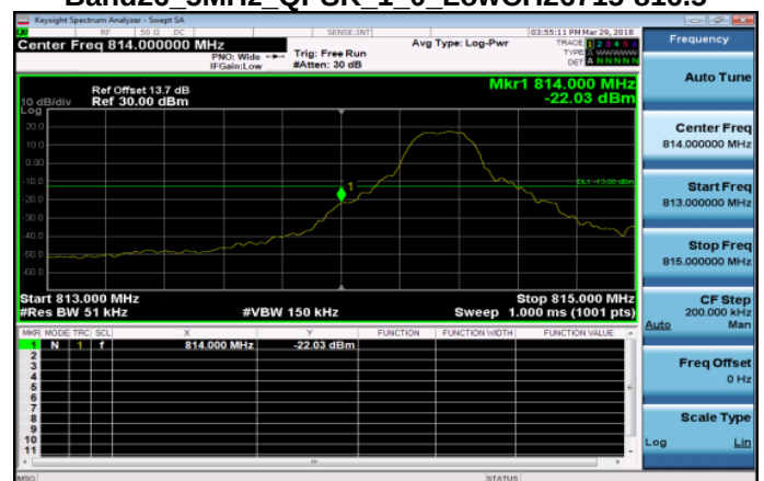
Band26_5MHz_QPSK_1_0_LowCH26715-816.5
