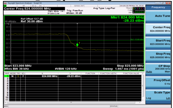
Band26_3MHz_QPSK_15_0_HighCH26775-822.5
