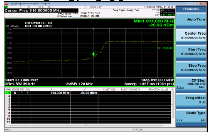
Band26_3MHz_QPSK_15_0_LowCH26705-815.5
