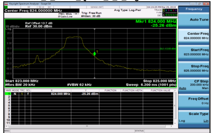
Band26_1_4MHz_QPSK_1_5_HighCH26783-823.3
