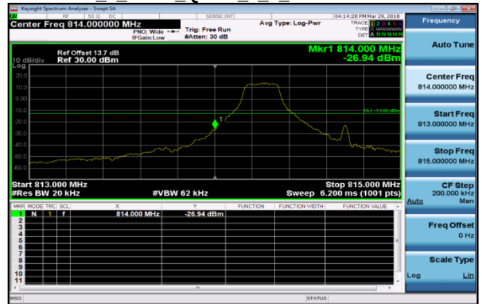
Band26_1_4MHz_QPSK_1_0_LowCH26697-814.7
