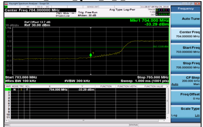
Band17 10MHz_QPSK_50_0_LowCH23780-709
