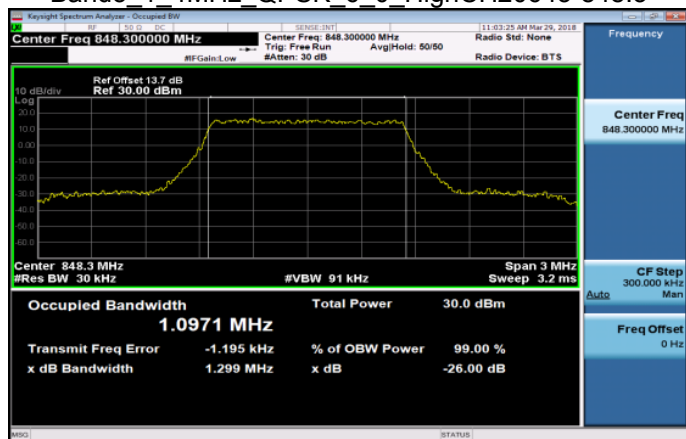
Band5_1_4MHz_QPSK_6_0_HighCH20643-848.3
