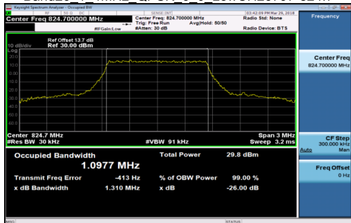
Band26_1_4MHz_QPSK_6_0_LowCH26797-824.7
