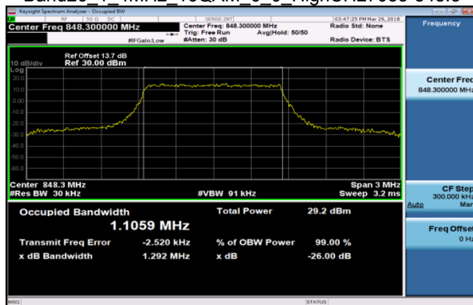
Band26_1_4MHz_16QAM_6_0_HighCH27033-848.3
