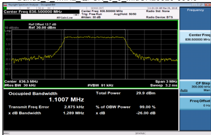
Band5_1_4MHz_QPSK_6_0_MidCH20525-836.5
