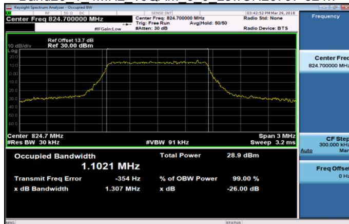
Band26_1_4MHz_16QAM_6_0_LowCH26797-824.7
