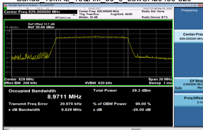
Band5_10MHz_16QAM_50_0_LowCH20450-829
