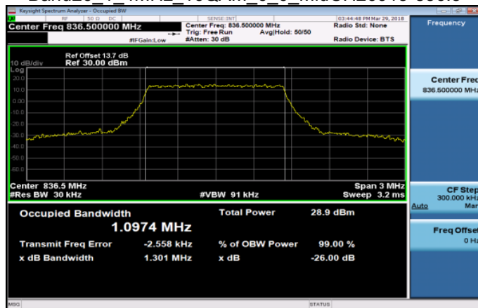
Band26_1_4MHz_16QAM_6_0_MidCH26915-836.5
