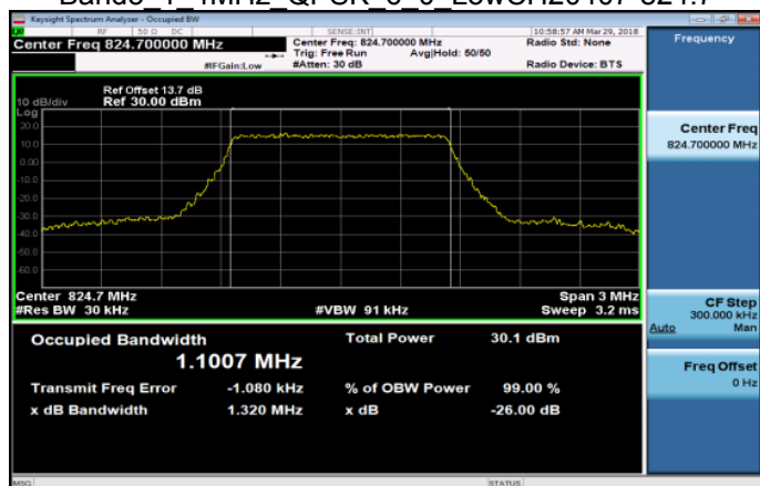
Band5_1_4MHz_QPSK_6_0_LowCH20407-824.7
