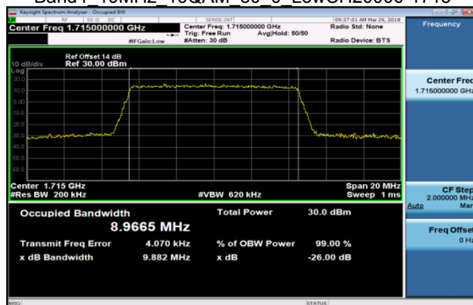
Band4_10MHz_16QAM_50_0_LowCH20000-1715
