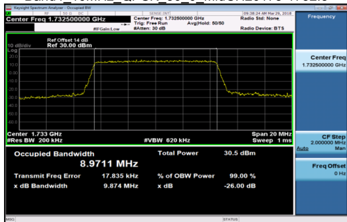
Band4_10MHz_QPSK_50_0_MidCH20175-1732.5
