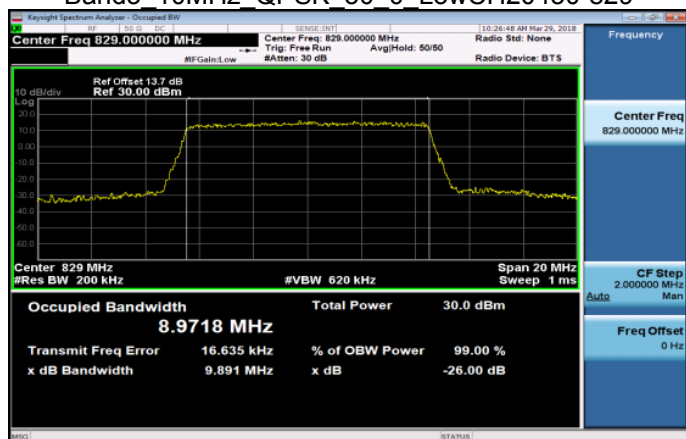
Band5_10MHz_QPSK_50_0_LowCH20450-829
