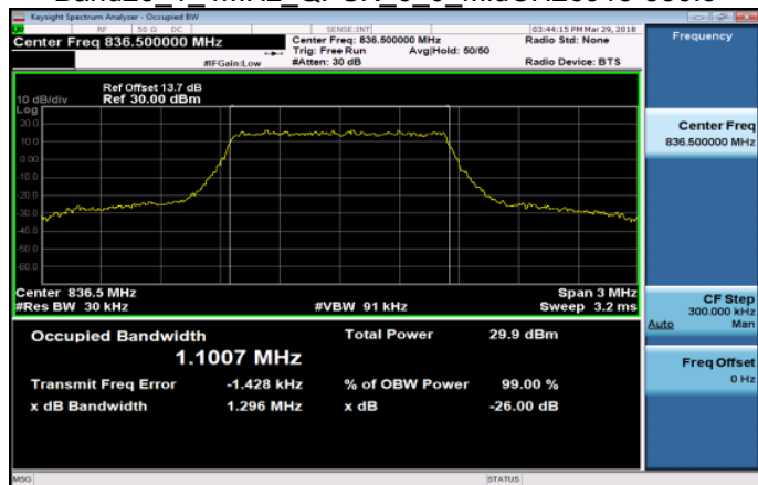
Band26_1_4MHz_QPSK_6_0_MidCH26915-836.5
