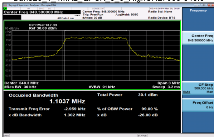
Band26_1_4MHz_QPSK_6_0_HighCH27033-848.3
