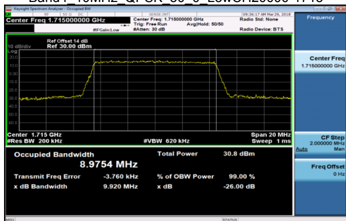
Band4_10MHz_QPSK_50_0_LowCH20000-1715
