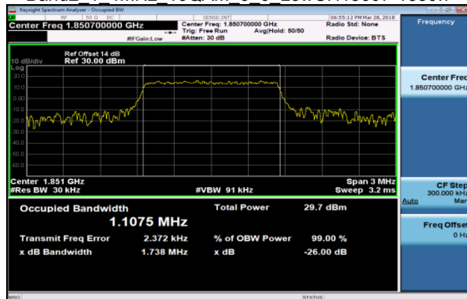
Band2_1_4MHz_16QAM_6_0_LowCH18607-1850.7
