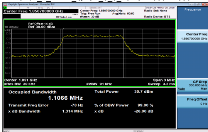
Band2_1_4MHz_QPSK_6_0_LowCH18607-1850.7
