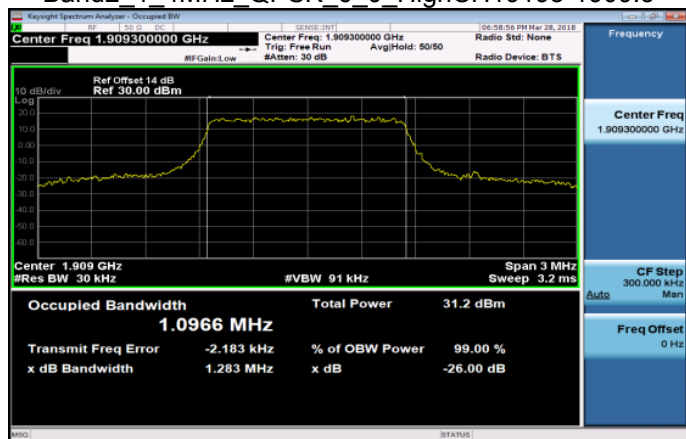
Band2_1_4MHz_QPSK_6_0_HighCH19193-1909.3
