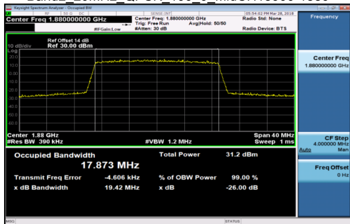
Band2_20MHz_QPSK_100_0_MidCH18900-1880
