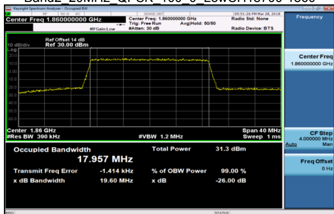
Band2_20MHz_QPSK_100_0_LowCH18700-1860
