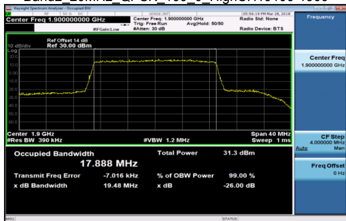
Band2_20MHz_QPSK_100_0_HighCH19100-1900
