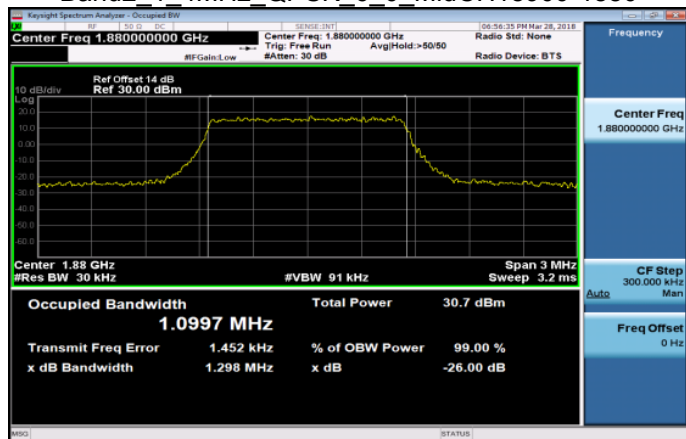
Band2_1_4MHz_QPSK_6_0_MidCH18900-1880
