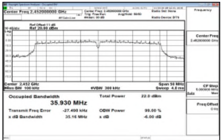
6dB Band Width Test Data CH-High (2452MHz)
