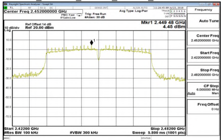
Reference Lev- el_802.11n_40MHz_Chain0_2452MHz
