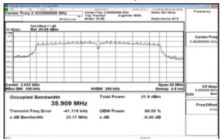
6dB Band Width Test Data CH-High (2452MHz)
