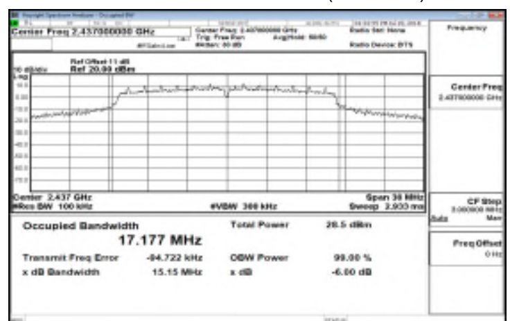
6dB Band Width Test Data CH-Mid (2437MHz)
