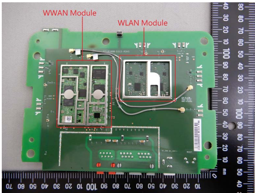
Internal View of EUT – 4 (Main PCB)
