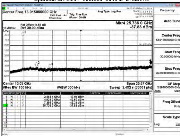
Spurious Emission 802.11b 20MHz 2462MHz
