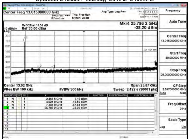
Spurious Emission 802.11g 20MHz 2462MHz
