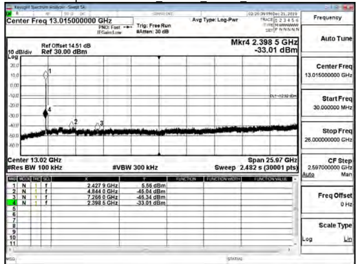
Spurious Emission 802.11n 40MHz 2437MHz
