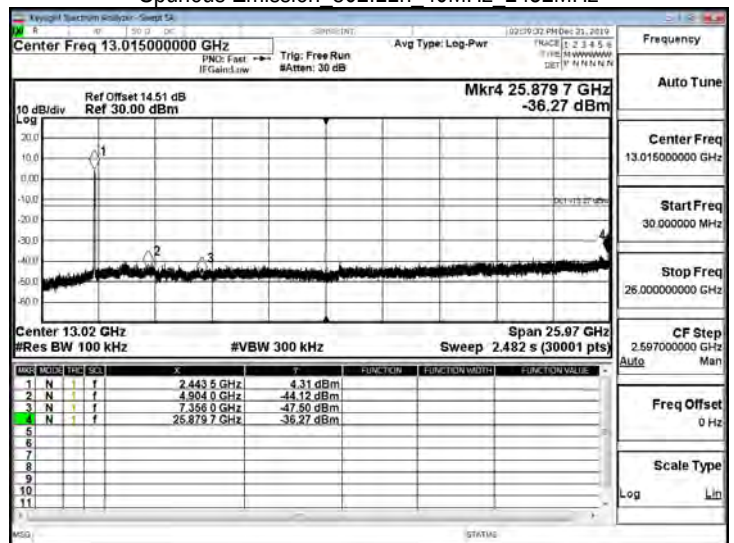
Spurious Emission 802.11n 40MHz 2452MHz
