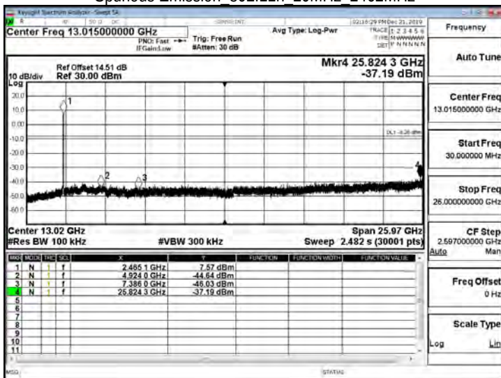
Spurious Emission 802.11n 20MHz 2462MHz
