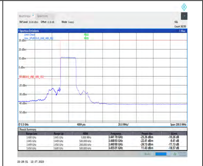
1-N77-3450-3550-PC1.5-30-20-L-3-DFT-PI2BPSK-Outer_Full-50@0-Ant3-1--PASS-see graph
