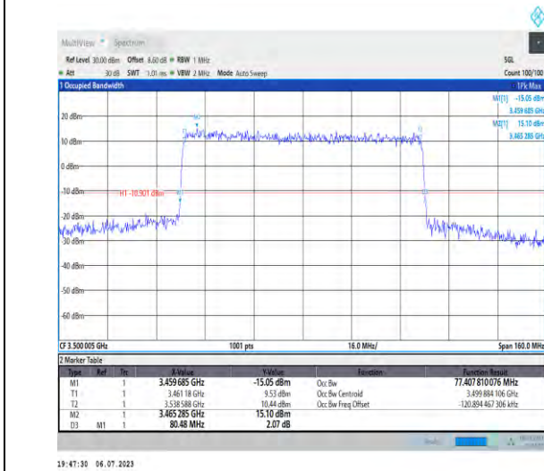
1-N77-3450-3550-PC1.5-30-80-M-7-CP-16QAM-Outer_Full-217@0-Ant3-77.408-80.480-≤80-PASS
