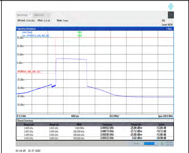
1-N77-3450-3550-PC1.5-30-40-L-6-CP-QPSK-Outer_Full-106@0-Ant3-1--PASS-see graph
