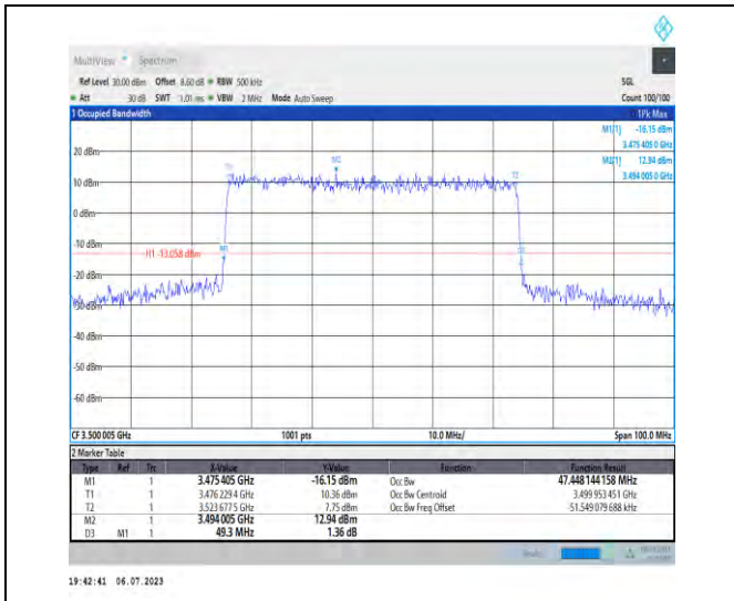
1-N77-3450-3550-PC1.5-30-50-M-7-CP-16QAM-Out er_Full-133@0-Ant3-47.448-49.300-≤50-PASS
