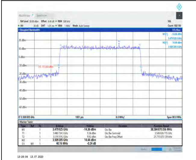
1-N77-3450-3550-PC1.5-30-40-M-6-CP-QPSK-Outer_Full-106@0-Ant3-38.585-40.160-≤40-PASS
