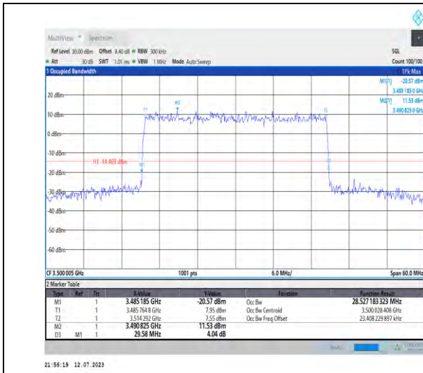
1-N77-3450-3550-PC1.5-30-30-M-5-DFT-256QAM-Outer_Full-75@0-Ant3-28.527-29.580-≤30-PASS
