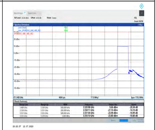
1-N77-3450-3550-PC1.5-30-15-H-6-CP-QPSK-Outer_Full-38@0-Ant3-1--PASS-see graph
