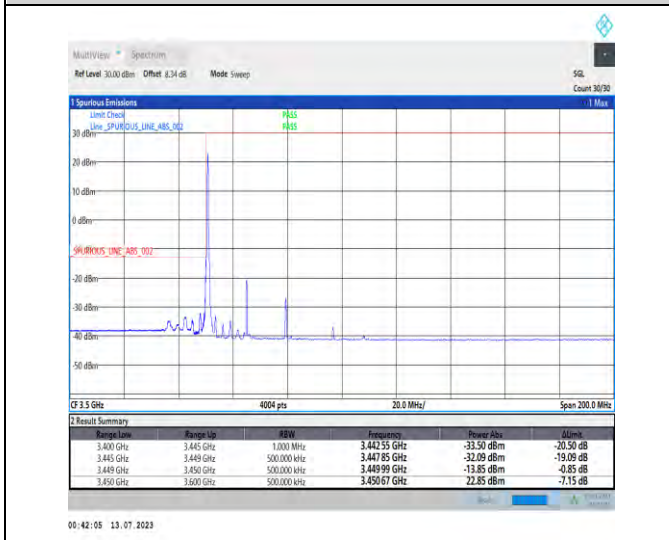
1-N77-3450-3550-PC1.5-30-30-L-4-CP-QPSK-Edge_1RB_Left-1@0-Ant3-1--PASS-see graph
