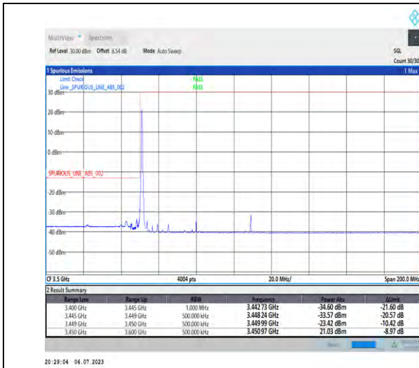
1-N77-3450-3550-PC1.5-30-60-L-1-DFT-PI2BPSK-Edge_1RB_Left-1@0-Ant3-1--PASS-see graph
