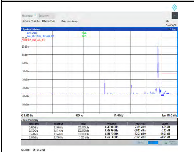
1-N77-3450-3550-PC1.5-30-60-H-5-CP-QPSK-Edge_1RB_Right-1@161-Ant3-1--PASS-see graph
