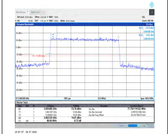
1-N77-3450-3550-PC1.5-30-80-M-8-CP-64QAM-Outer_Full-217@0-Ant3-77.754-80.640-≤80-PASS
