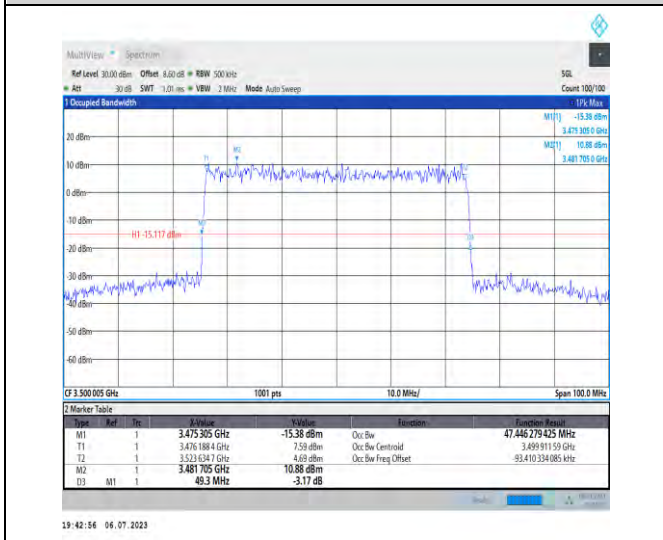
1-N77-3450-3550-PC1.5-30-50-M-9-CP-256QAM-Out er_Full-133@0-Ant3-47.446-49.300-≤50-PASS
