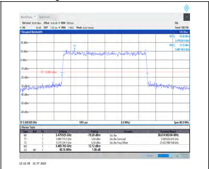
1-N77-3450-3550-PC1.5-30-40-M-9-CP-256QAM-Outer_Full-106@0-Ant3-38.630-40.160-≤40-PASS
