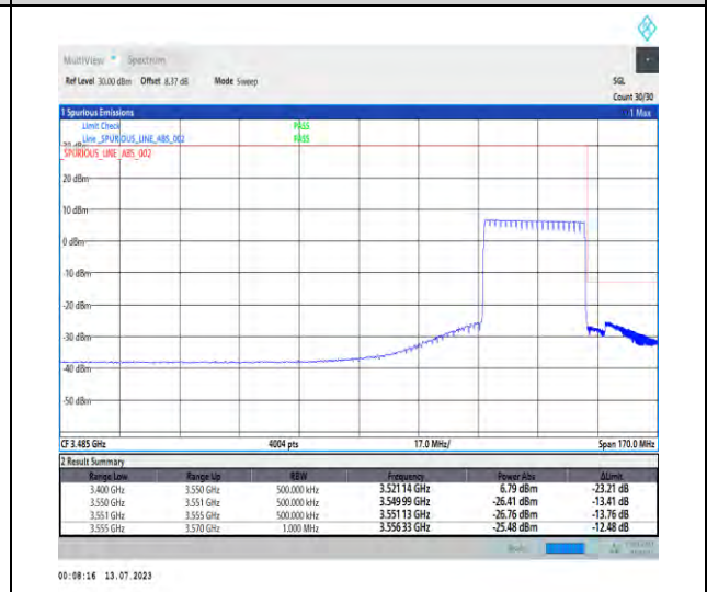
1-N77-3450-3550-PC1.5-30-30-H-6-CP-QPSK-Outer_Full-75@0-Ant3-1--PASS-see graph
