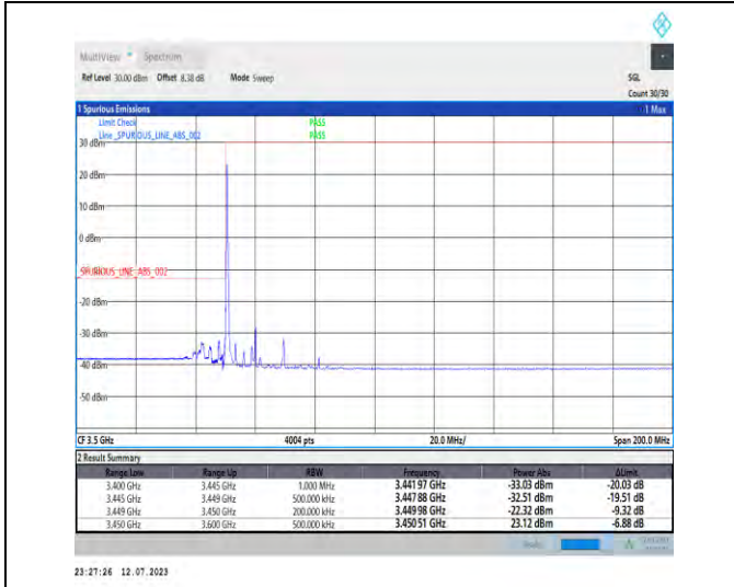
1-N77-3450-3550-PC1.5-30-20-L-1-DFT-PI2BPSK-Edge_1RB_Left-1@0-Ant3-1--PASS-see graph
