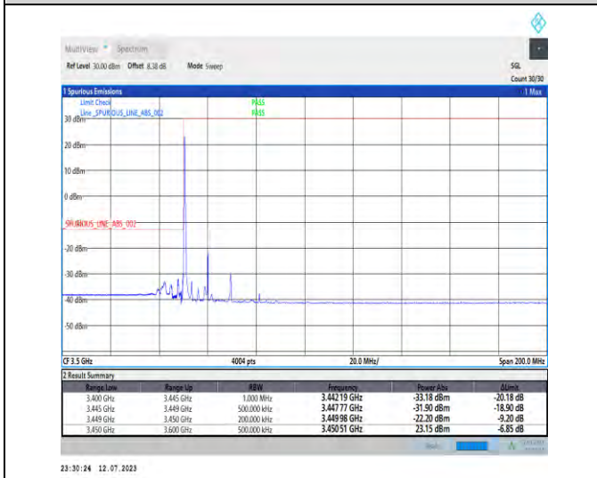
1-N77-3450-3550-PC1.5-30-20-L-4-CP-QPSK-Edge_1RB_Left-1@0-Ant3-1--PASS-see graph
