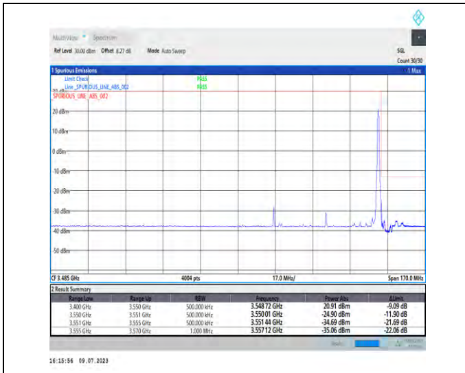
1-N77-3450-3550-PC1.5-30-50-H-2-DFT-PI2BPSK-Edge_1RB_Right-1@132-Ant3-1--PASS-see graph
