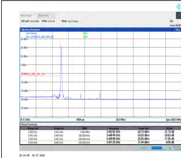
1-N77-3450-3550-PC1.5-30-50-L-1-DFT-PI2BPSK-Edge_1RB_Left-1@0-Ant3-1--PASS-see graph
