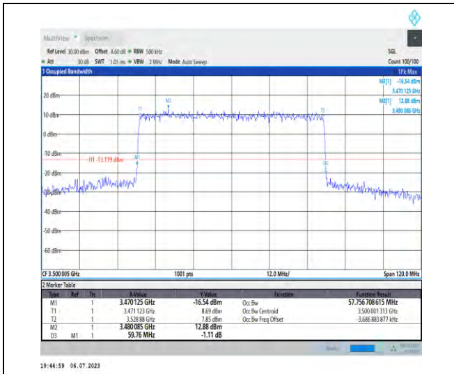
1-N77-3450-3550-PC1.5-30-60-M-6-CP-QPSK-Outer_Full-162@0-Ant3-57.757-59.760-≤60-PASS
