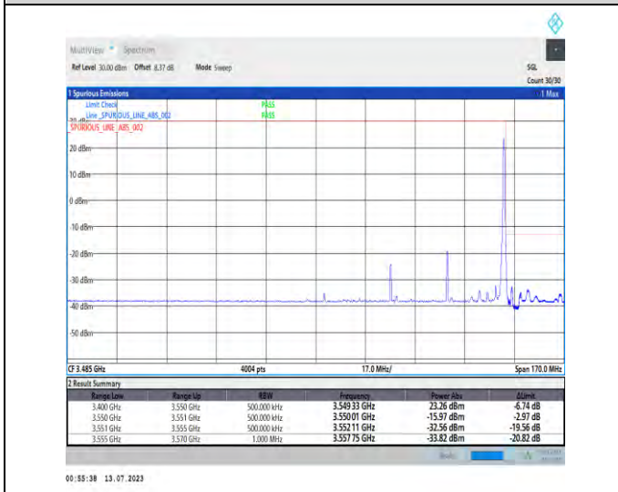
1-N77-3450-3550-PC1.5-30-40-H-5-CP-QPSK-Edge_1RB_Right-1@105-Ant3-1--PASS-see graph
