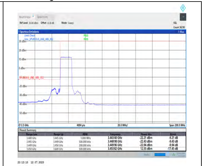
1-N77-3450-3550-PC1.5-30-15-L-3-DFT-PI2BPSK-Outer_Full-36@0-Ant3-1--PASS-see graph
