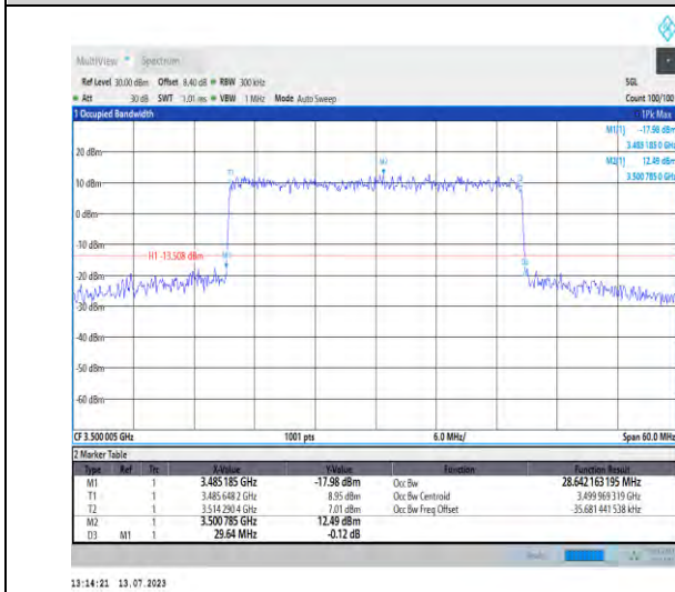
1-N77-3450-3550-PC1.5-30-30-M-7-CP-16QAM-Outer_Full-75@0-Ant3-28.642-29.640-≤30-PASS
