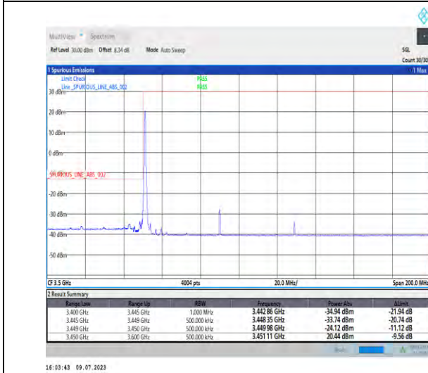
1-N77-3450-3550-PC1.5-30-80-L-4-CP-QPSK-Edge_1RB_Left-1@0-Ant3-1--PASS-see graph
