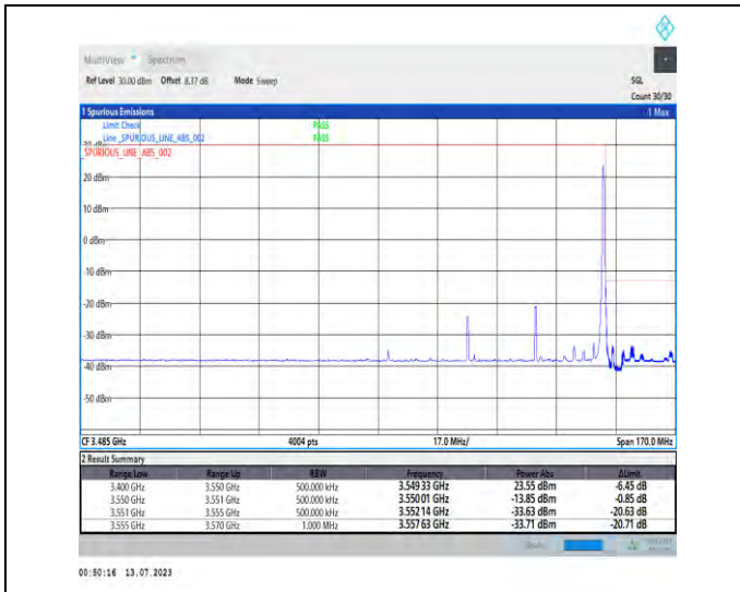
1-N77-3450-3550-PC1.5-30-40-H-2-DFT-PI2BPSK-Edge_1RB_Right-1@105-Ant3-1--PASS-see graph
