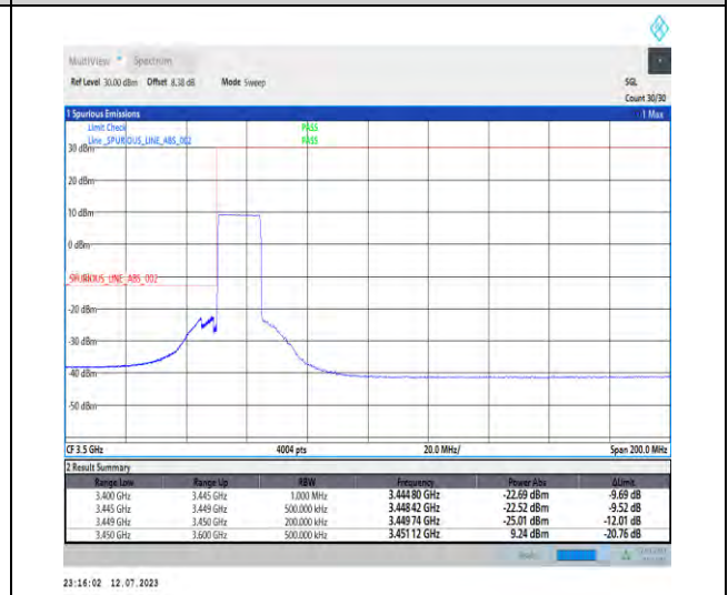
1-N77-3450-3550-PC1.5-30-15-L-6-CP-QPSK-Outer_Full-38@0-Ant3-1--PASS-see graph
