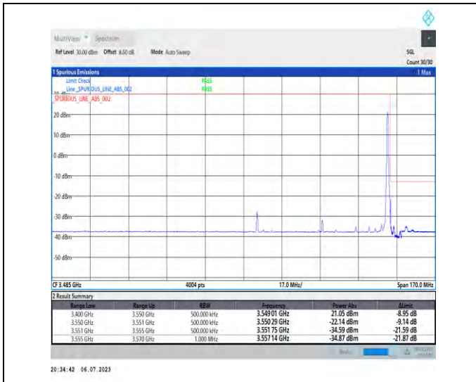
1-N77-3450-3550-PC1.5-30-60-H-2-DFT-PI2BPSK-Edge_1RB_Right-1@161-Ant3-1--PASS-see graph
