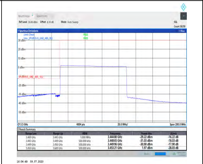
1-N77-3450-3550-PC1.5-30-80-L-6-CP-QPSK-Outer_Full-217@0-Ant3-1--PASS-see graph
