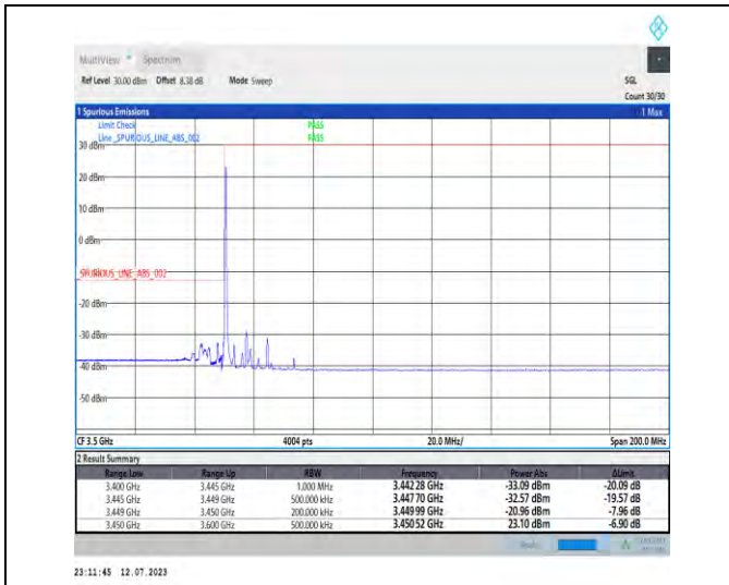
1-N77-3450-3550-PC1.5-30-15-L-1-DFT-PI2BPSK-Edge_1RB_Left-1@0-Ant3-1--PASS-see graph
