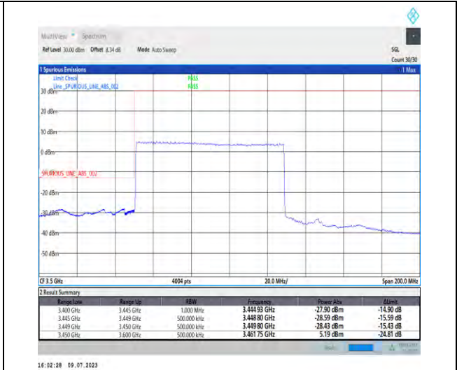
1-N77-3450-3550-PC1.5-30-80-L-3-DFT-PI2BPSK-Outer_Full-100@0-Ant3-1--PASS-see graph
