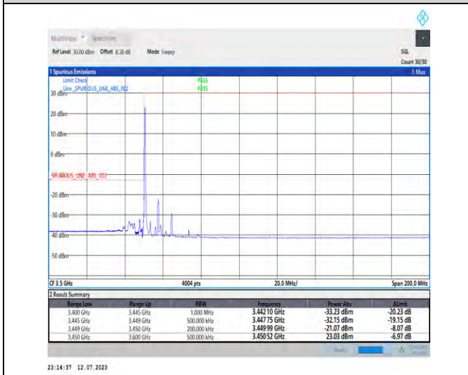
1-N77-3450-3550-PC1.5-30-15-L-4-CP-QPSK-Edge_1RB_Left-1@0-Ant3-1--PASS-see graph
