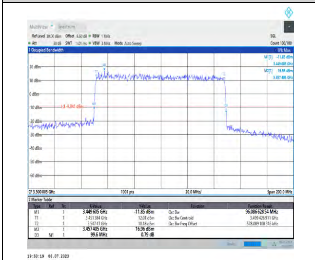
1-N77-3450-3550-PC1.5-30-100-M-1-DFT-QPSK-Outer_Full-270@0-Ant3-96.087-99.600-≤100-PASS
