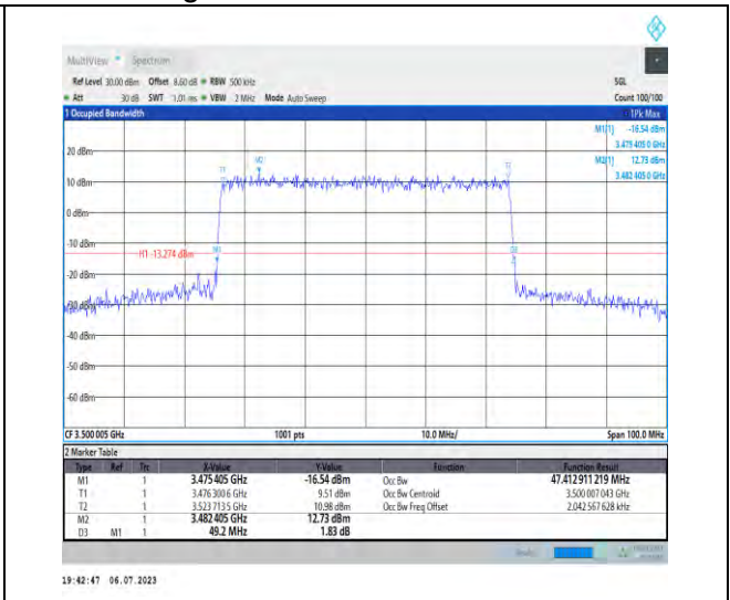
1-N77-3450-3550-PC1.5-30-50-M-8-CP-64QAM-Out er_Full-133@0-Ant3-47.413-49.200-≤50-PASS
