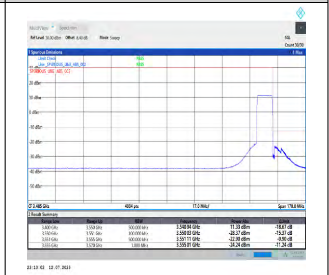
1-N77-3450-3550-PC1.5-30-10-H-6-CP-QPSK-Outer_Full-24@0-Ant3-1--PASS-see graph
