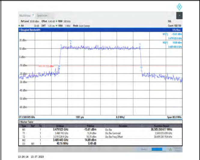
1-N77-3450-3550-PC1.5-30-40-M-7-CP-16QAM-Outer_Full-106@0-Ant3-38.585-40.160-≤40-PASS
