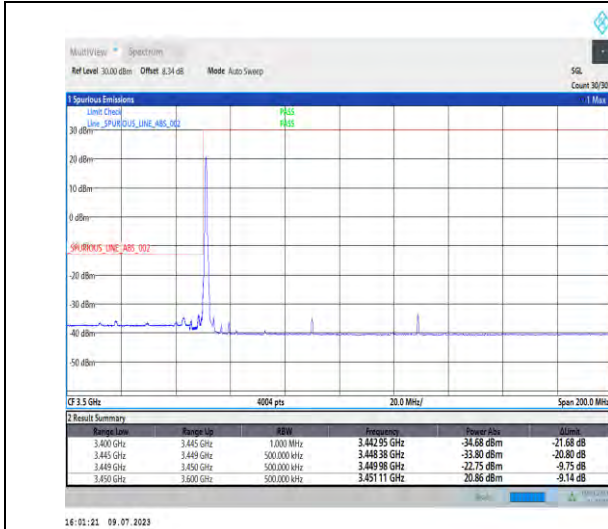
1-N77-3450-3550-PC1.5-30-80-L-1-DFT-PI2BPSK-Edge_1RB_Left-1@0-Ant3-1--PASS-see graph
