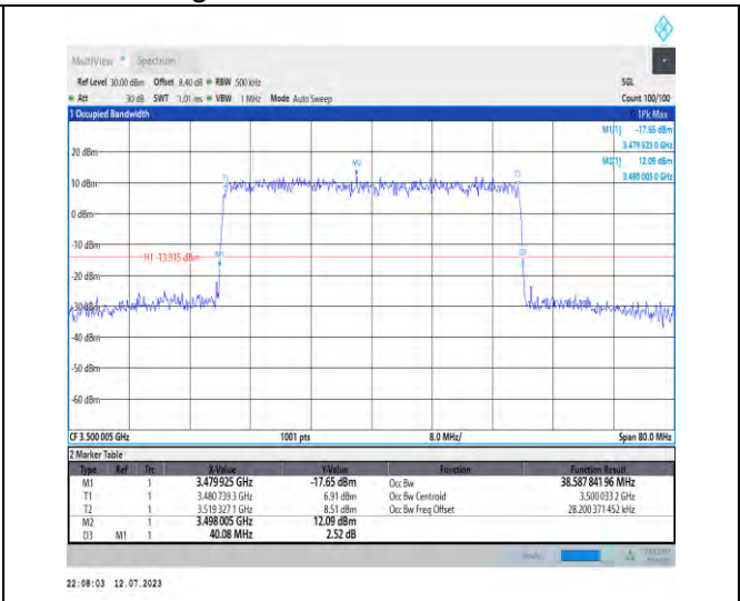
1-N77-3450-3550-PC1.5-30-40-M-5-DFT-256QAM-Outer_Full-100@0-Ant3-38.588-40.080-≤40-PASS
