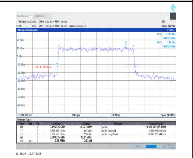
1-N77-3450-3550-PC1.5-30-10-M-8-CP-64QAM-Outer_Full-24@0-Ant3-9.318-9.760-≤10-PASS
