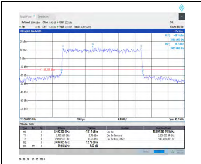
1-N77-3450-3550-PC1.5-30-20-M-7-CP-16QAM-Out er_Full-51@0-Ant3-18.898-19.640-≤20-PASS
