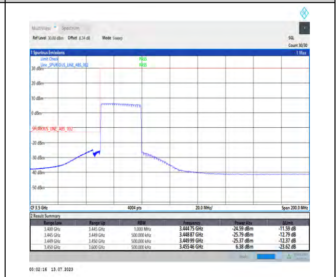
1-N77-3450-3550-PC1.5-30-30-L-6-CP-QPSK-Outer_Full-75@0-Ant3-1--PASS-see graph
