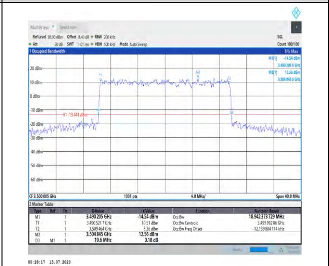
1-N77-3450-3550-PC1.5-30-20-M-6-CP-QPSK-Outer_Full-51@0-Ant3-18.942-19.600-≤20-PASS
