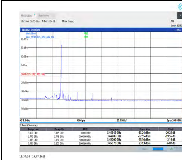
1-N77-3450-3550-PC1.5-30-40-L-1-DFT-PI2BPSK-Edge_1RB_Left-1@0-Ant3-1--PASS-see graph
