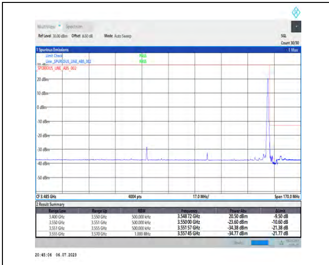
1-N77-3450-3550-PC1.5-30-80-H-2-DFT-PI2BPSK-Edge_1RB_Right-1@216-Ant3-1--PASS-see graph
