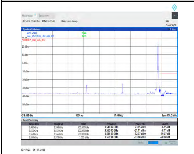
1-N77-3450-3550-PC1.5-30-80-H-5-CP-QPSK-Edge_1RB_Right-1@216-Ant3-1--PASS-see graph
