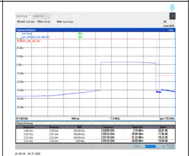
1-N77-3450-3550-PC1.5-30-60-H-6-CP-QPSK-Outer_Full-162@0-Ant3-1--PASS-see graph
