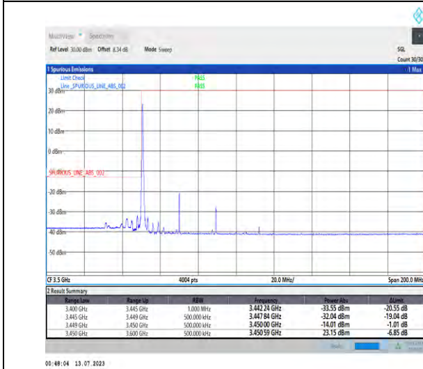
1-N77-3450-3550-PC1.5-30-40-L-4-CP-QPSK-Edge_1RB_Left-1@0-Ant3-1--PASS-see graph
