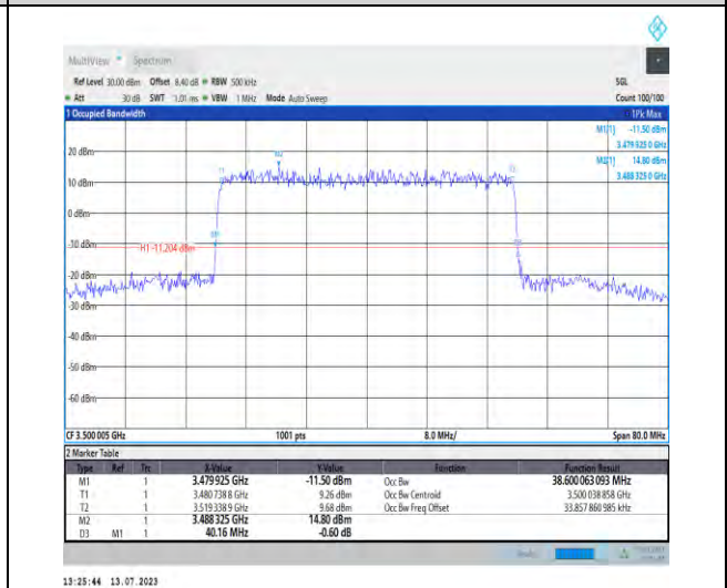
1-N77-3450-3550-PC1.5-30-40-M-3-DFT-16QAM-O uter_Full-100@0-Ant3-38.6-40.160-≤40-PASS
