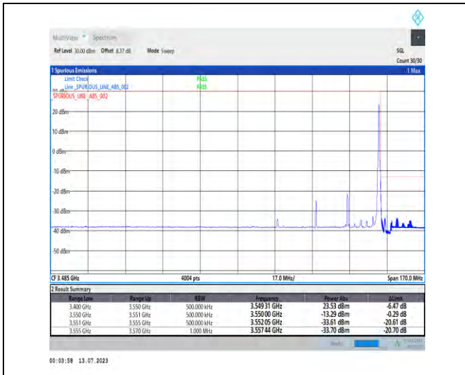
1-N77-3450-3550-PC1.5-30-30-H-2-DFT-PI2BPSK-Edge_1RB_Right-1@77-Ant3-1--PASS-see graph
