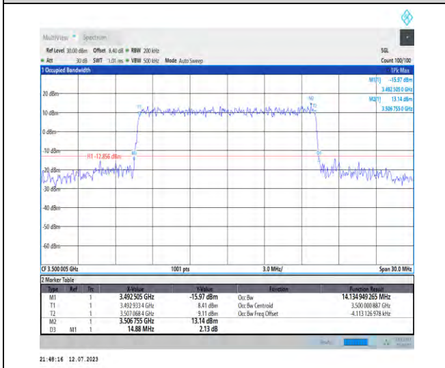
1-N77-3450-3550-PC1.5-30-15-M-6-CP-QPSK-Outer_Full-38@0-Ant3-14.135-14.880-≤30-PASS
