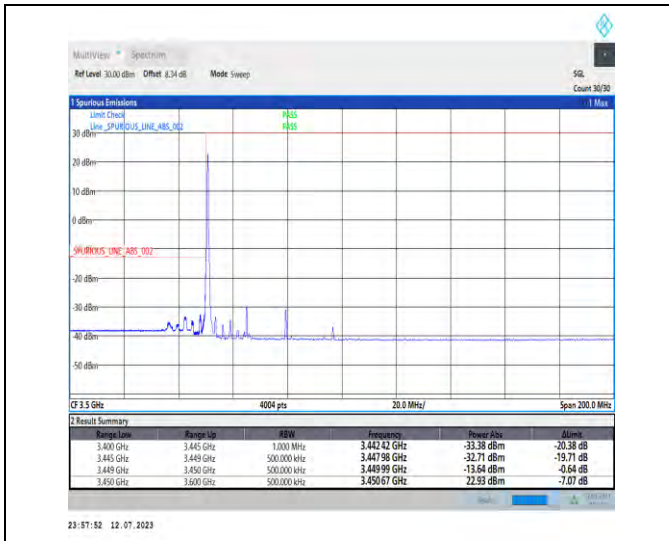
1-N77-3450-3550-PC1.5-30-30-L-1-DFT-PI2BPSK-Edge_1RB_Left-1@0-Ant3-1--PASS-see graph
