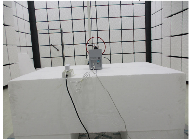
Part_15.247_BLE_Radiated_Setup
