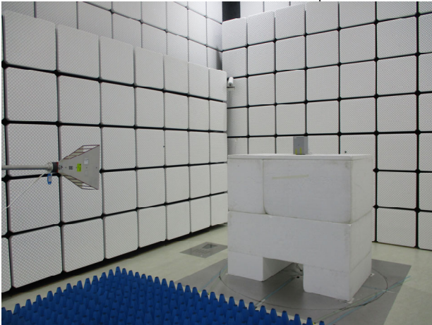
Part_15.247_BLE_Radiated_Setup
