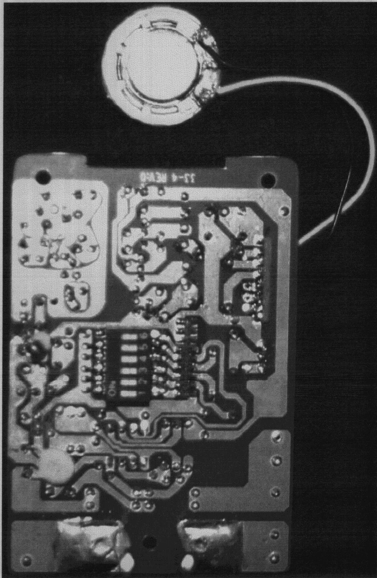
Photo 4. Receiver Board, Solder Side
