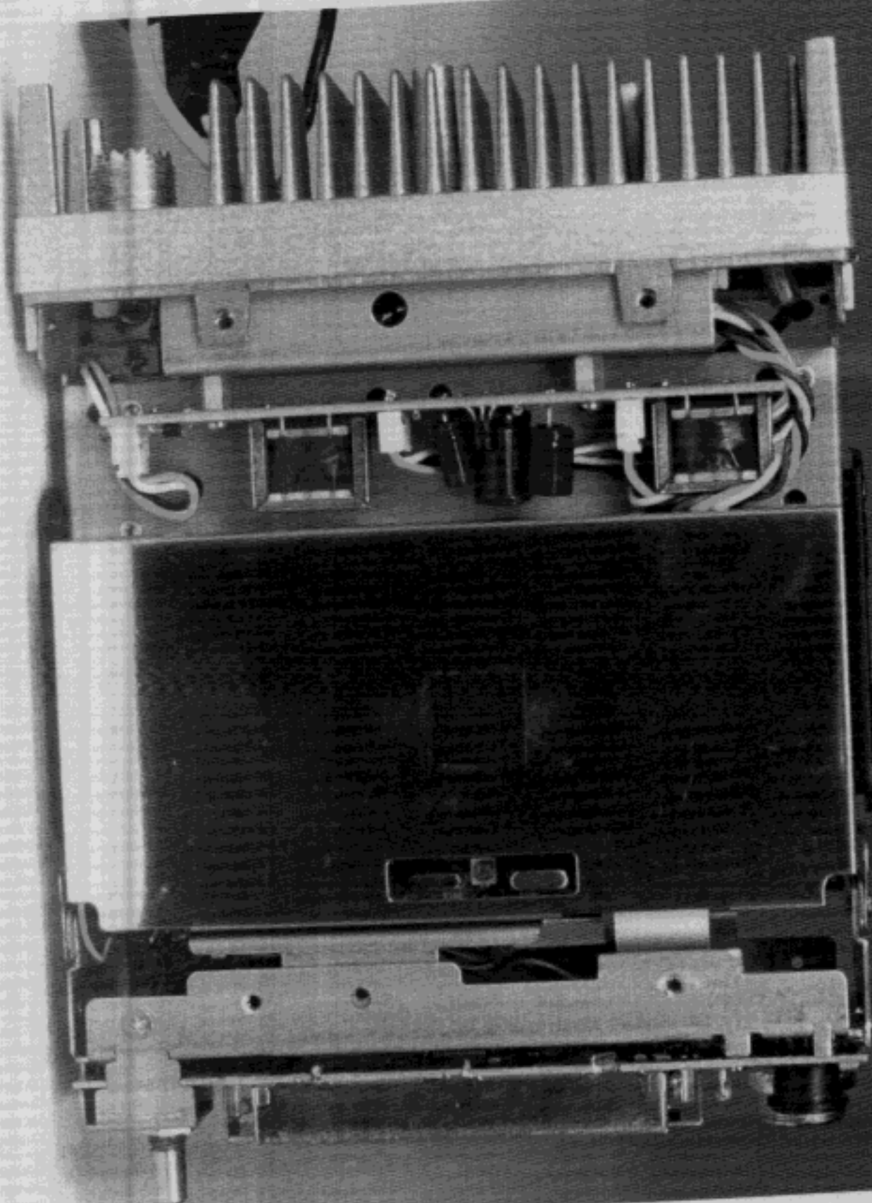
8R00924 FCC ID: H7CM-10A TAD Radio of Canada Inc. M10 Mobile Radio with 10W & 30W Power Output Interior View, Bottom Side
