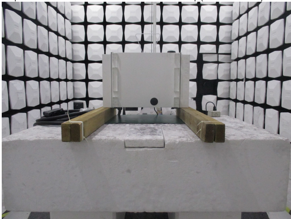
Description : Front View of Radiated Emission Test Setup (30 MHz ~ 1 GHz)
